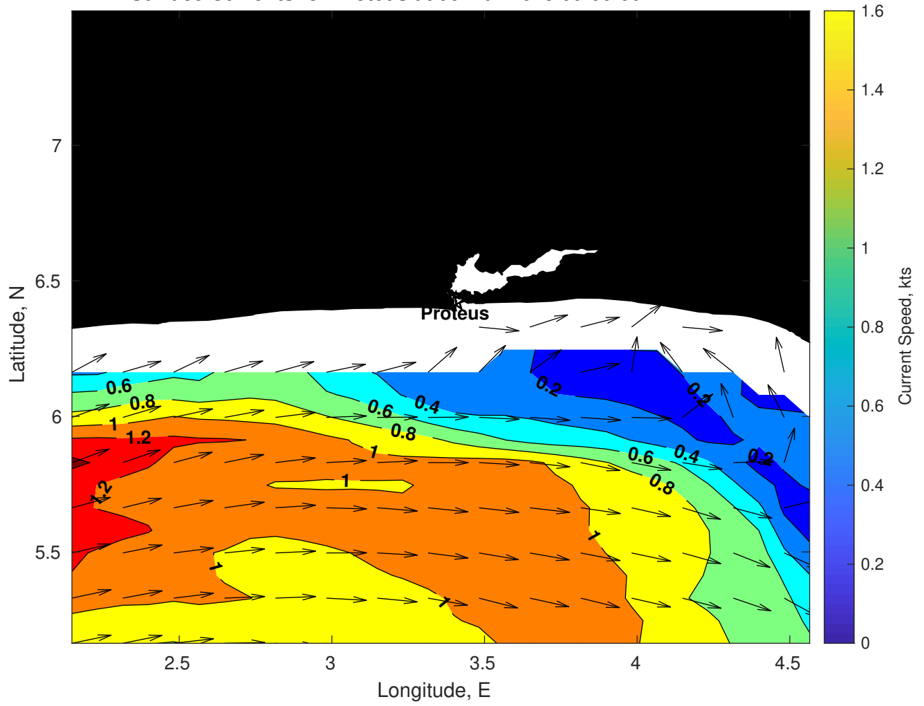
Surface Currents for Proteus at 06-Mar-2025 00:00:00
