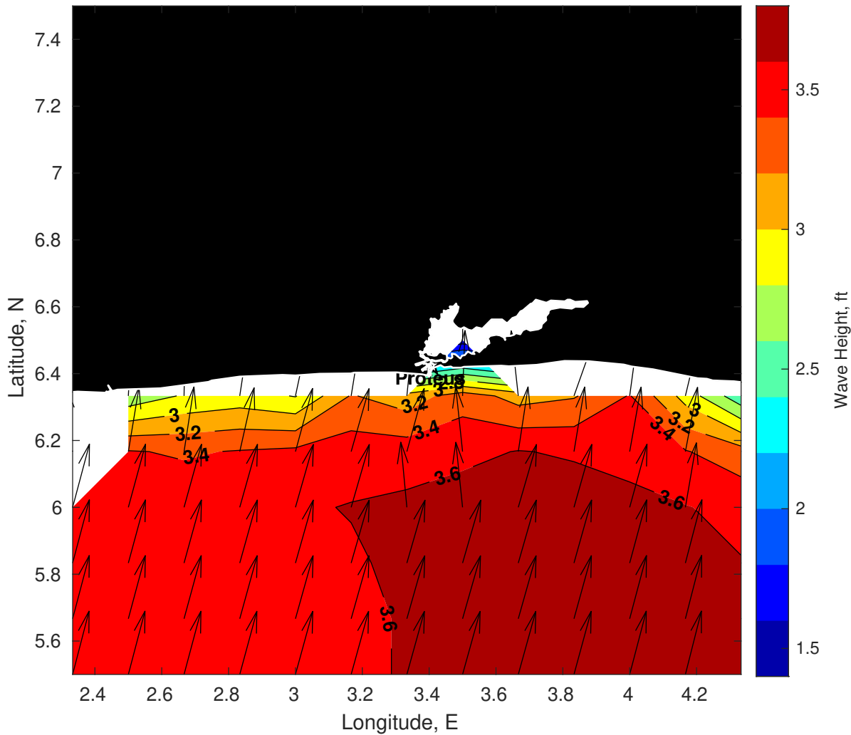
Wave Height (ft) for Proteus at 07-Mar-2025 09:00:00
