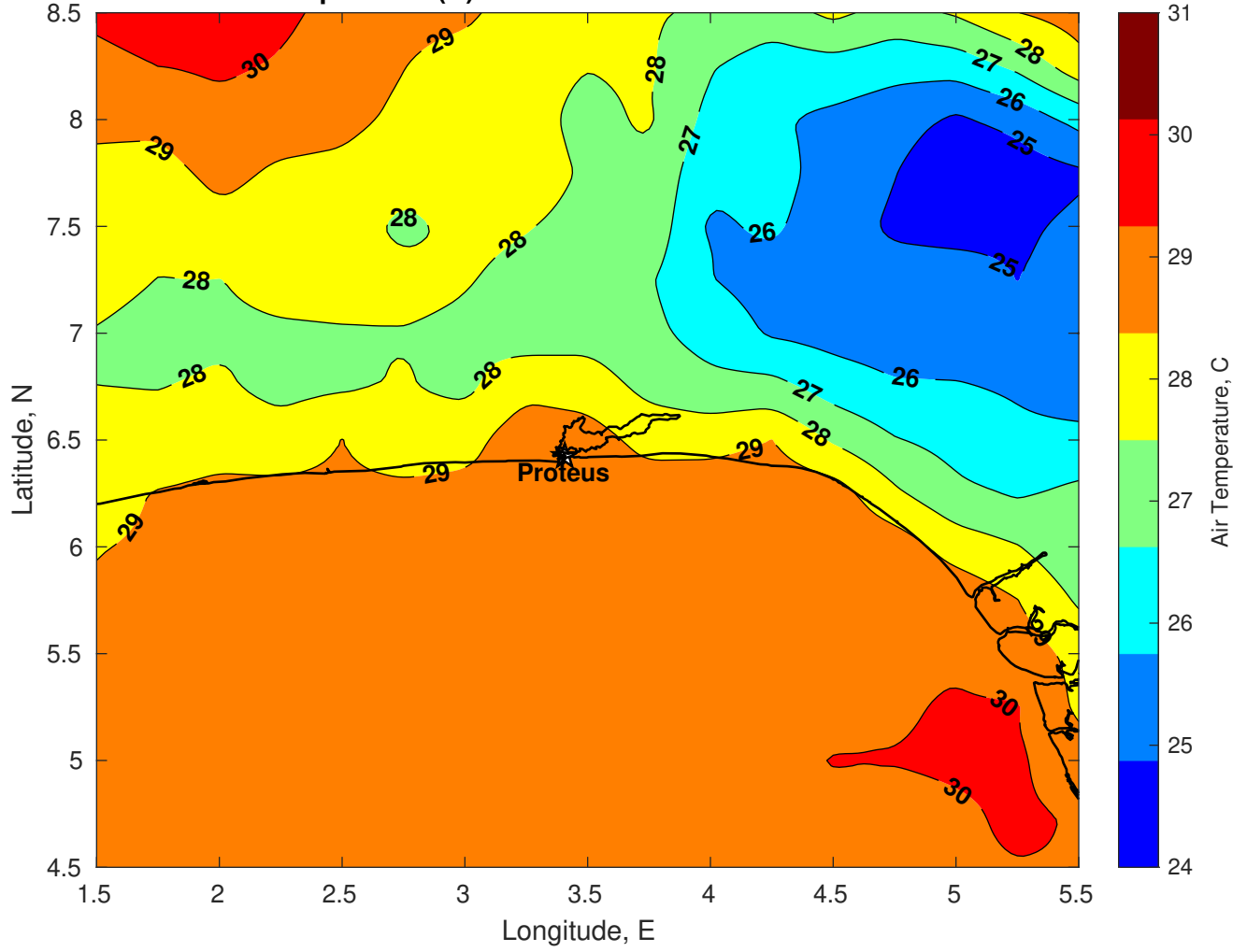
Air Temperature (C) for Proteus at 07-Mar-2025
