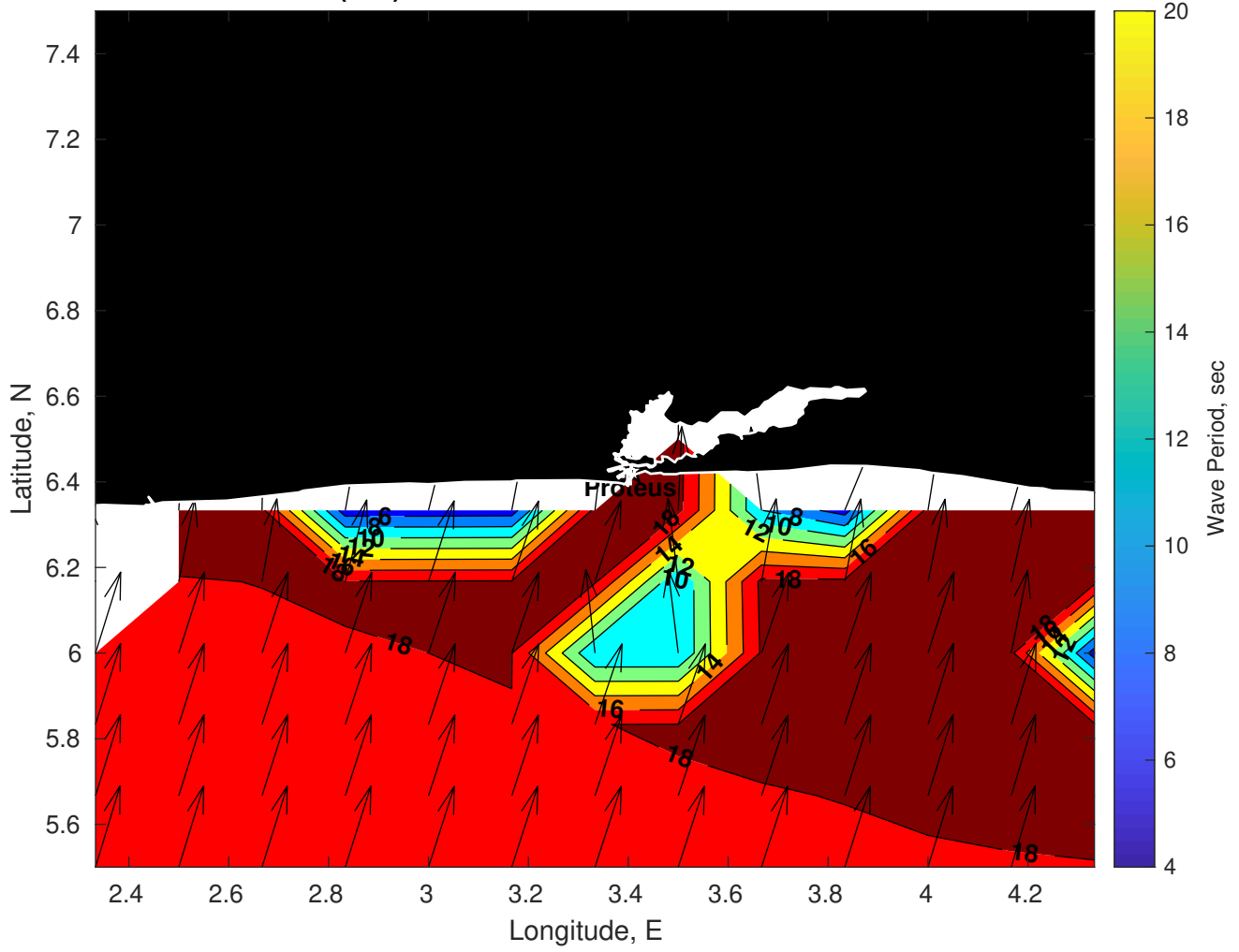
Wave Period (sec) for Proteus at 07-Mar-2025 09:00:00
