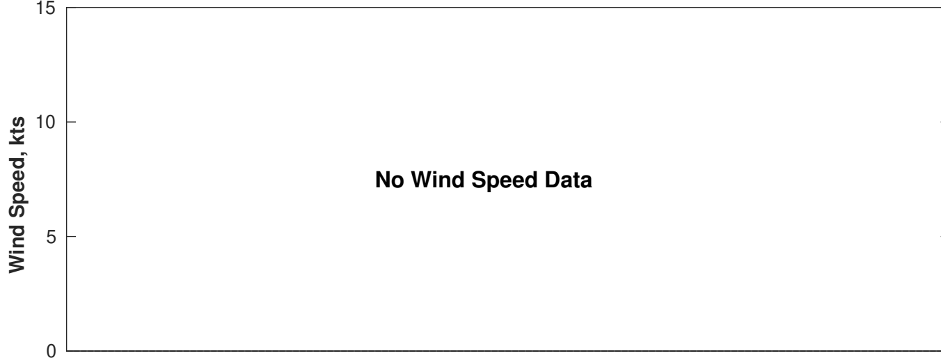
Wind & Wave Forecast for Proteus from 07-Mar-2025 01:00:00 to 23-Mar-2025 01:00:00
