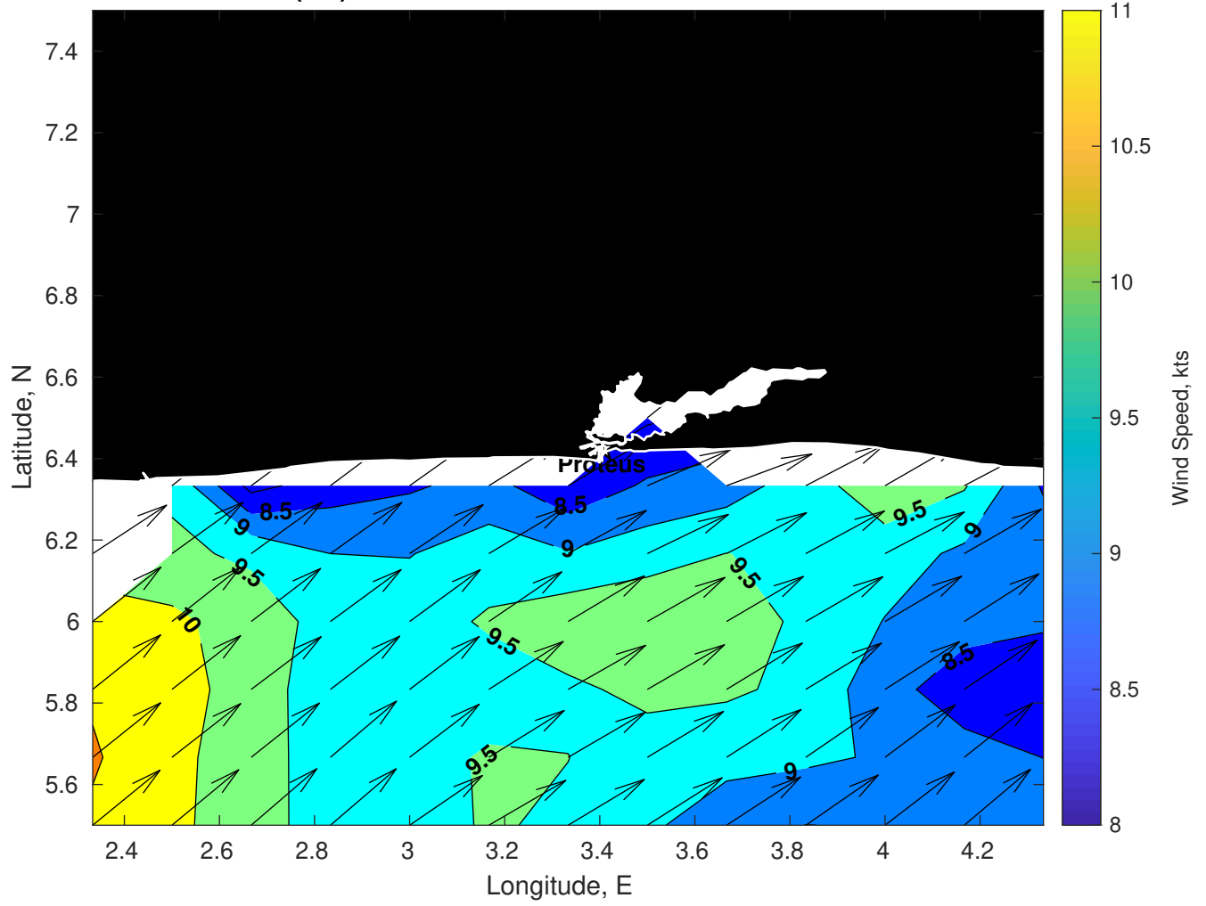
Winds (kts) for Proteus at 07-Mar-2025 09:00:00
