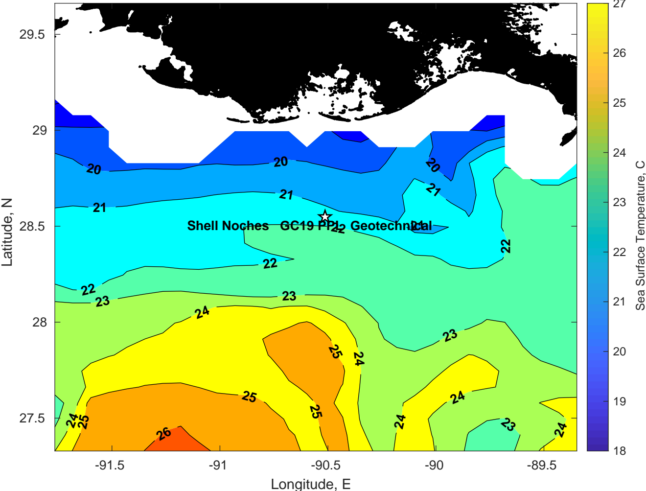
SST for Shell Noches GC19 PPL Geotechnical at 05-Mar-2025 00:00:00
