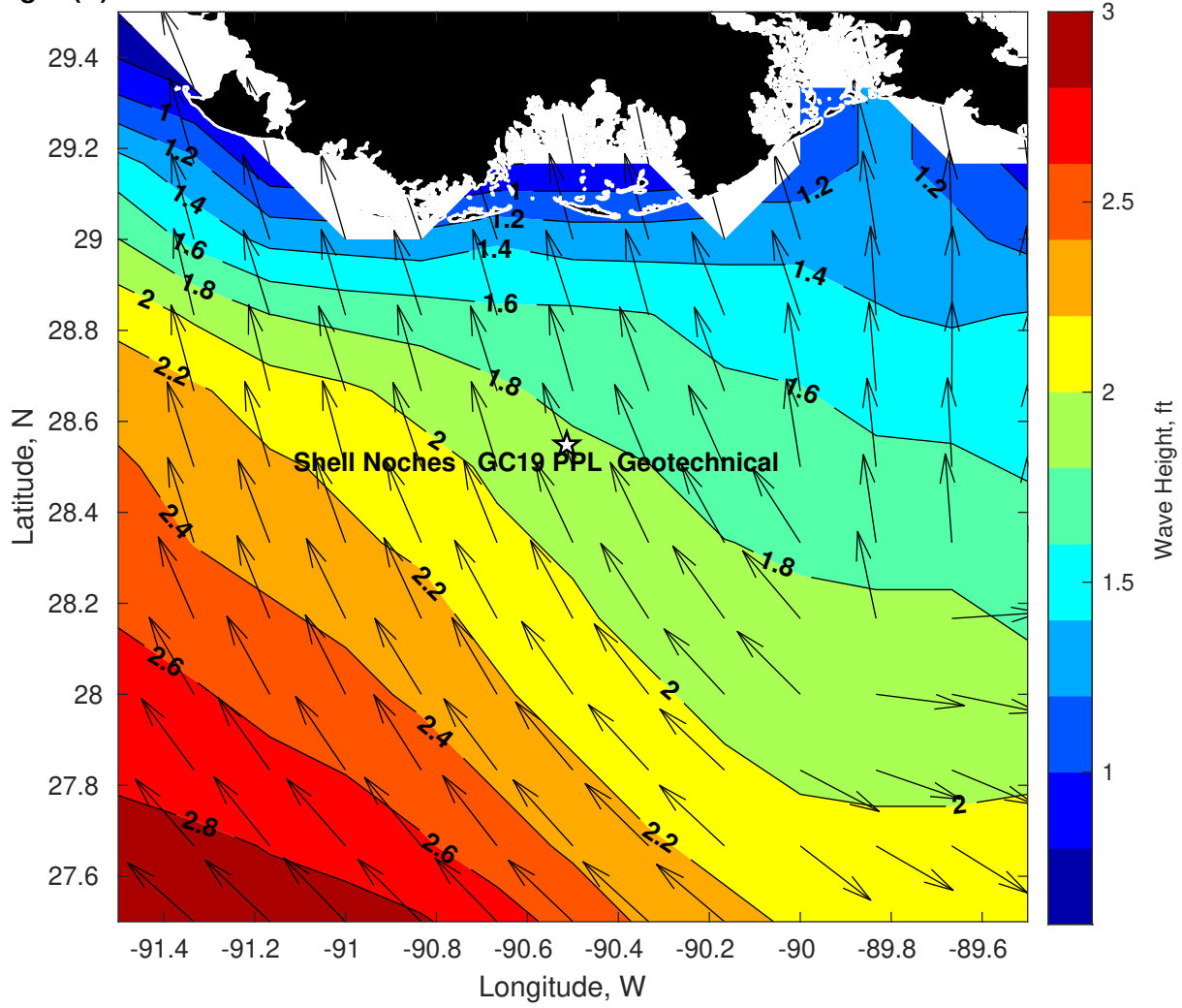
Wave Height (ft) for Shell Noches GC19 PPL Geotechnical at 07-Mar-2025 09:00:00
