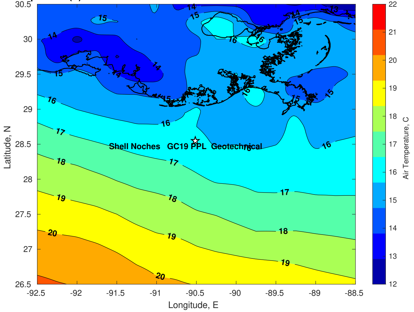
Air Temperature (C) for Shell Noches GC19 PPL Geotechnical at 07-Mar-2025
