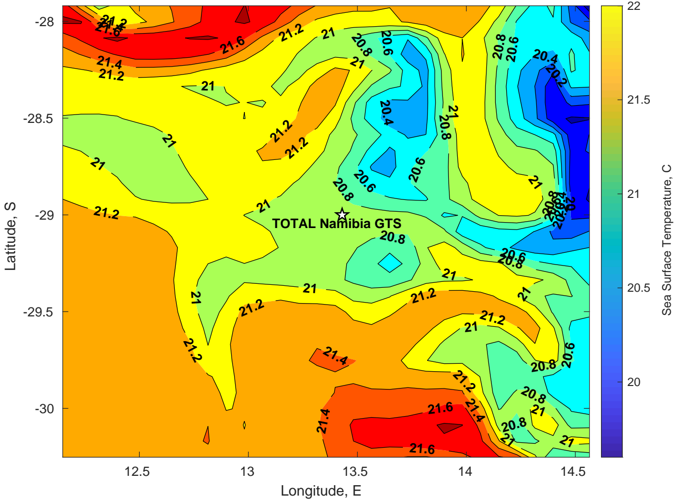
SST for TOTAL Namibia GTS at 05-Mar-2025 00:00:00
