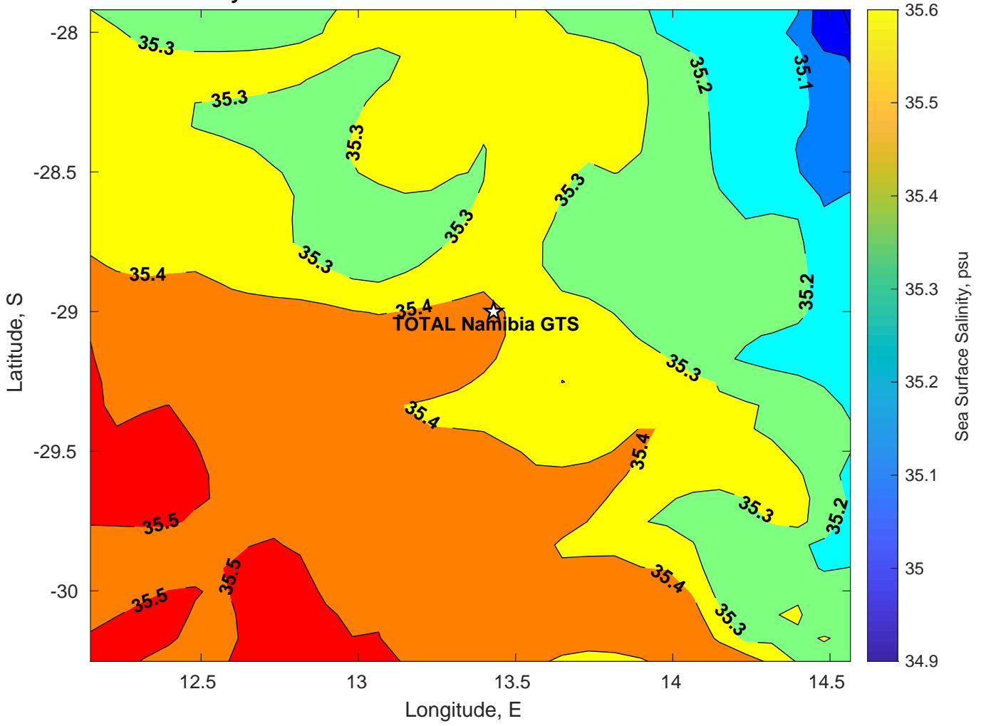
Surface Salinity for TOTAL Namibia GTS at 05-Mar-2025 00:00:00
