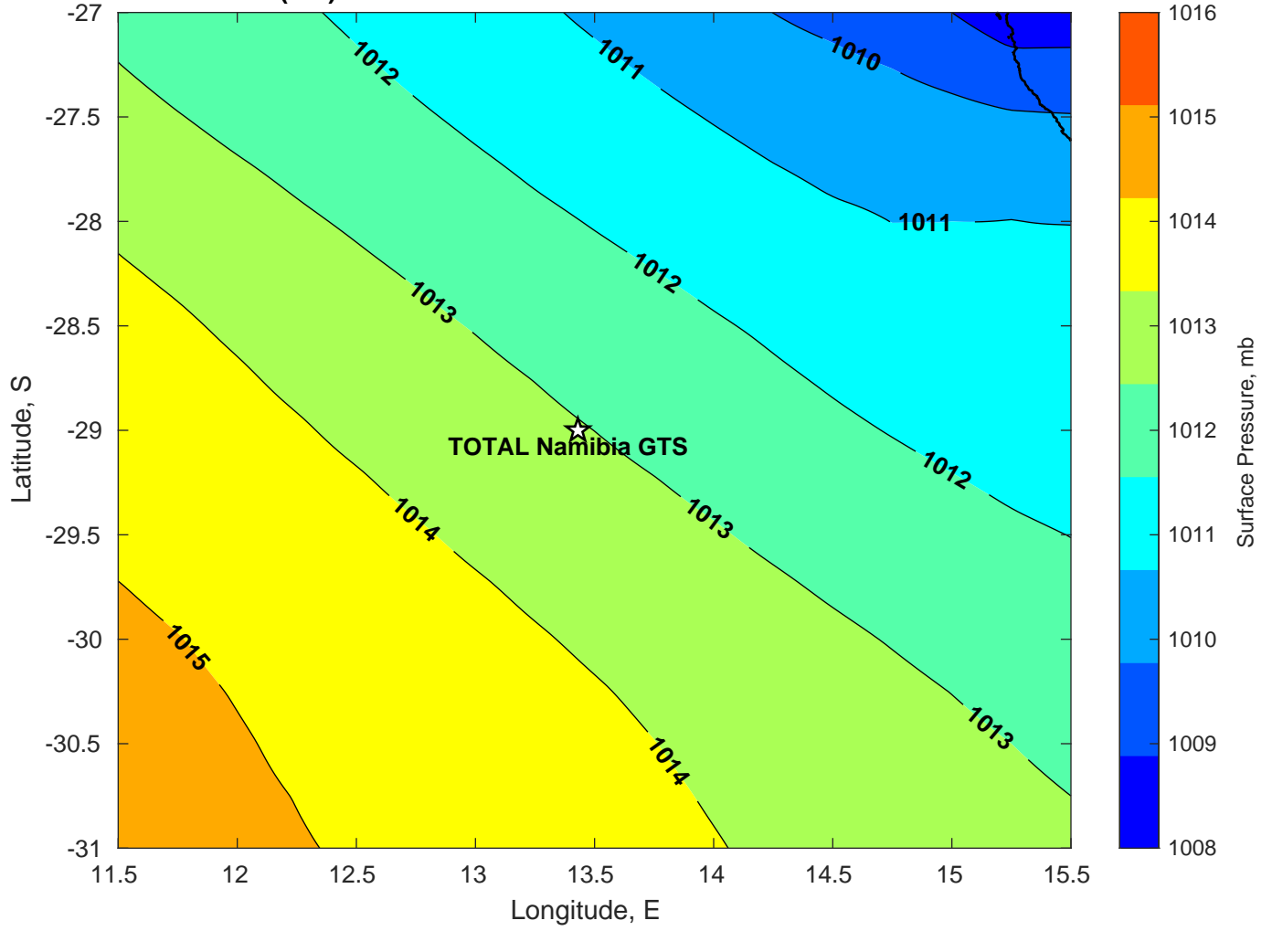
Surface Pressure (mb) for TOTAL Namibia GTS at 09-Mar-2025 00:00:00
