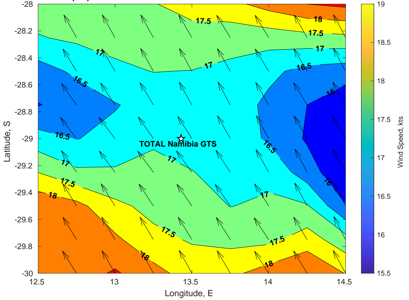
Winds (kts) for TOTAL Namibia GTS at 07-Mar-2025 09:00:00
