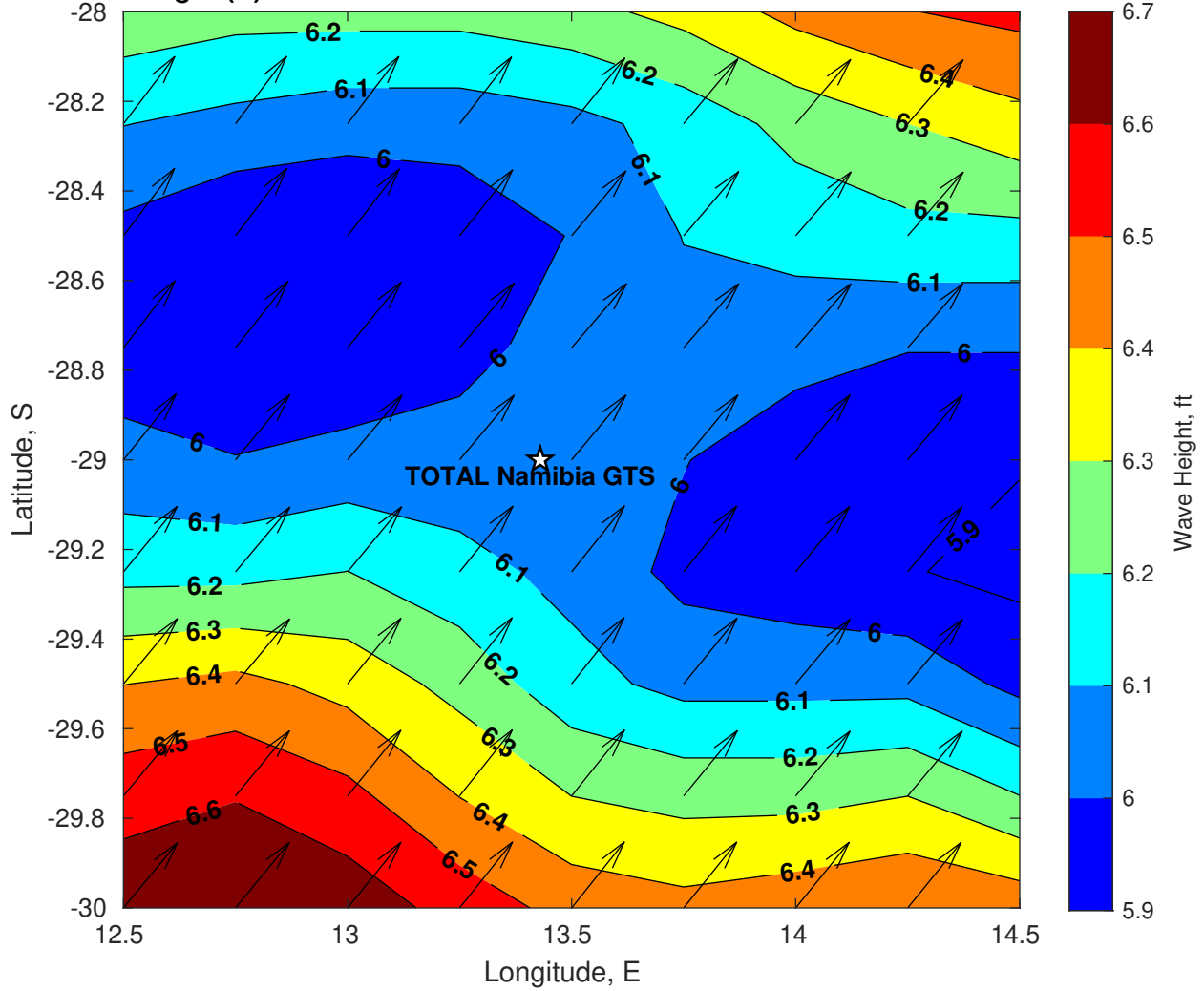
Wave Height (ft) for TOTAL Namibia GTS at 07-Mar-2025 09:00:00
