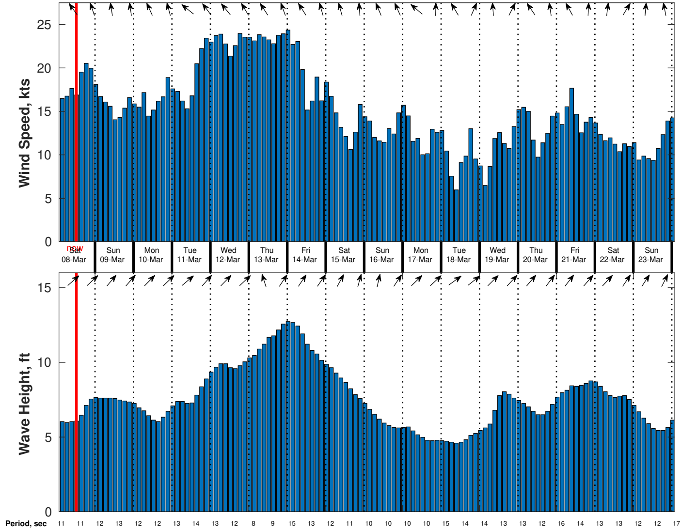
Wind & Wave Forecast for TOTAL Namibia GTS from 07-Mar-2025 02:00:00 to 23-Mar-2025 02:00:00
