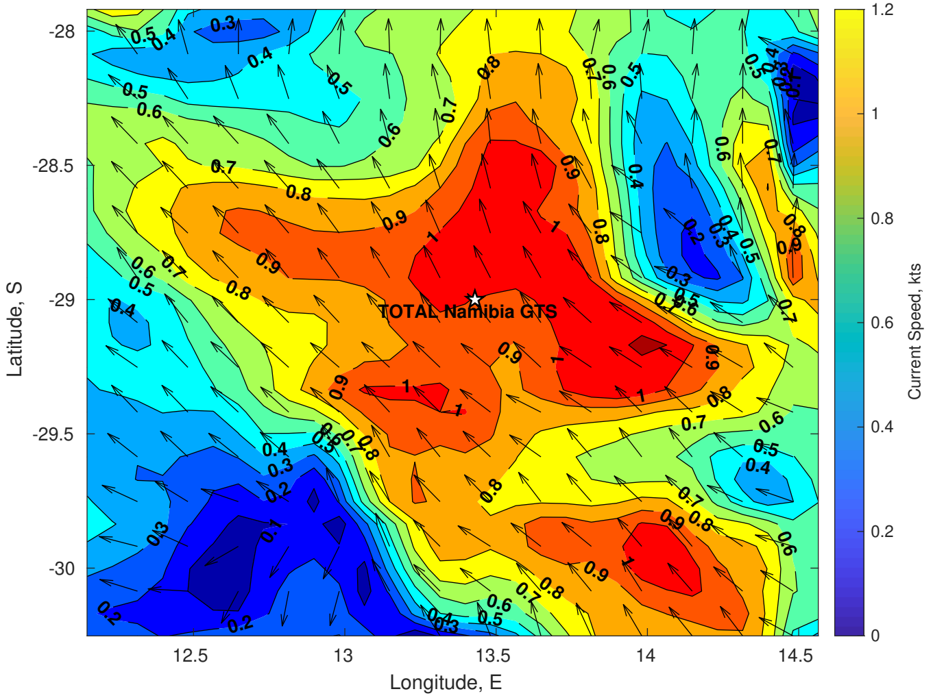
Surface Currents for TOTAL Namibia GTS at 05-Mar-2025 00:00:00
