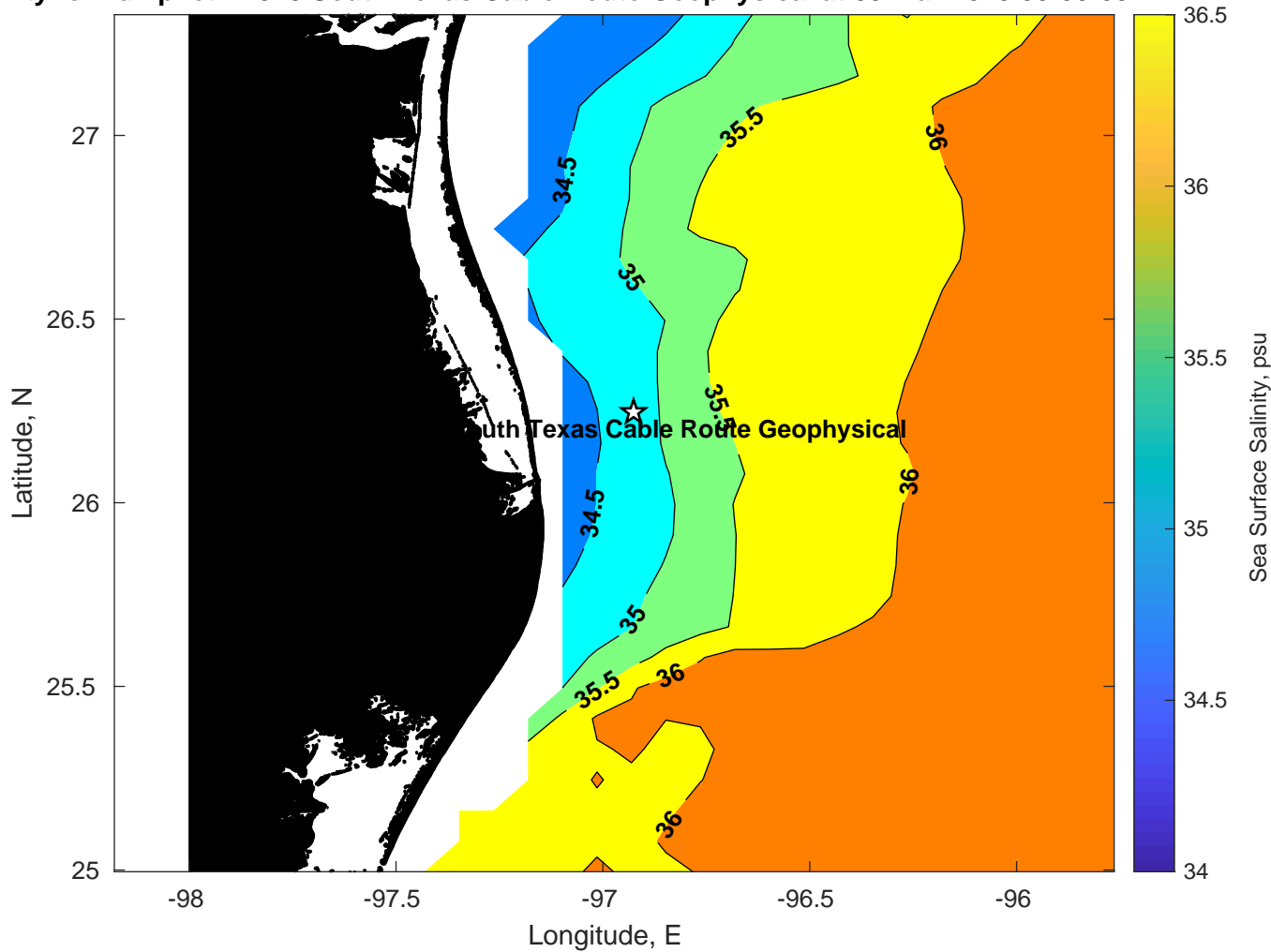
Surface Salinity for Tampnet P2378 South Texas Cable Route Geophysical at 05-Mar-2025 00:00:00
