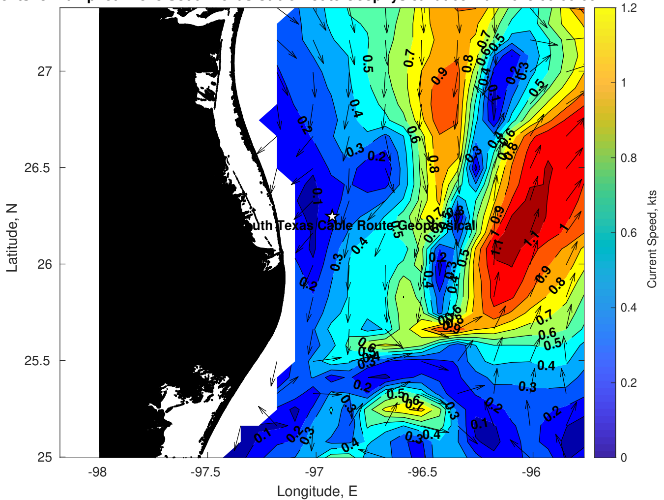
Surface Currents for Tampnet P2378 South Texas Cable Route Geophysical at 05-Mar-2025 00:00:00
