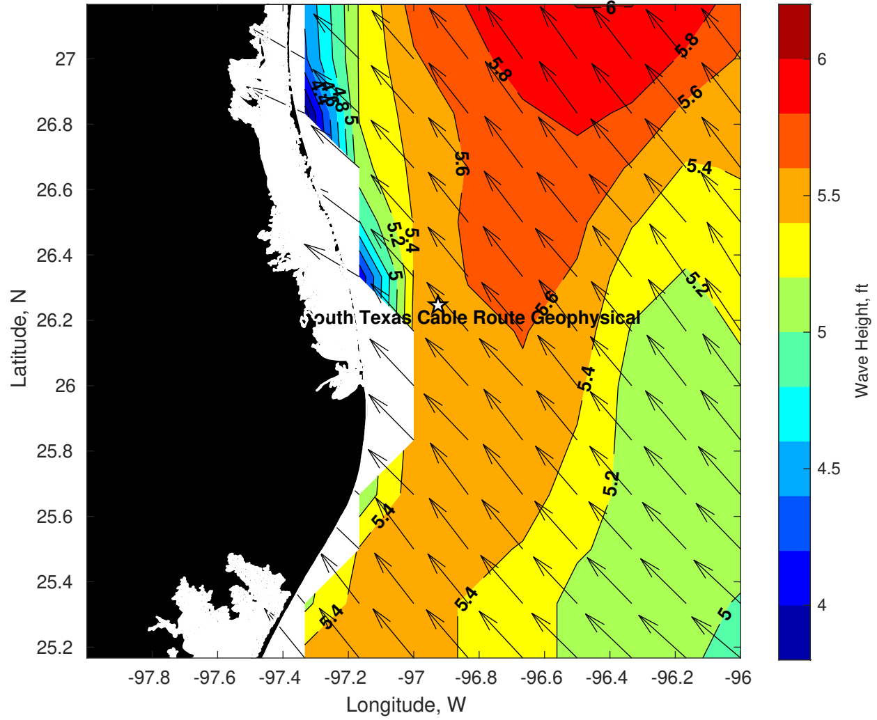
Wave Height (ft) for Tampnet P2378 South Texas Cable Route Geophysical at 07-Mar-2025 09:00:00
