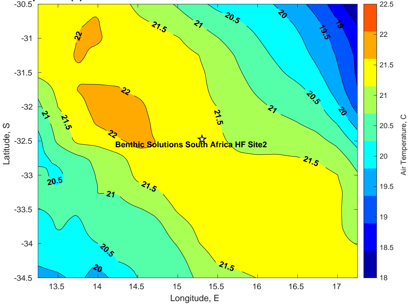
Air Temperature (C) for Benthic Solutions South Africa HF Site2 at 08-Mar-2025
