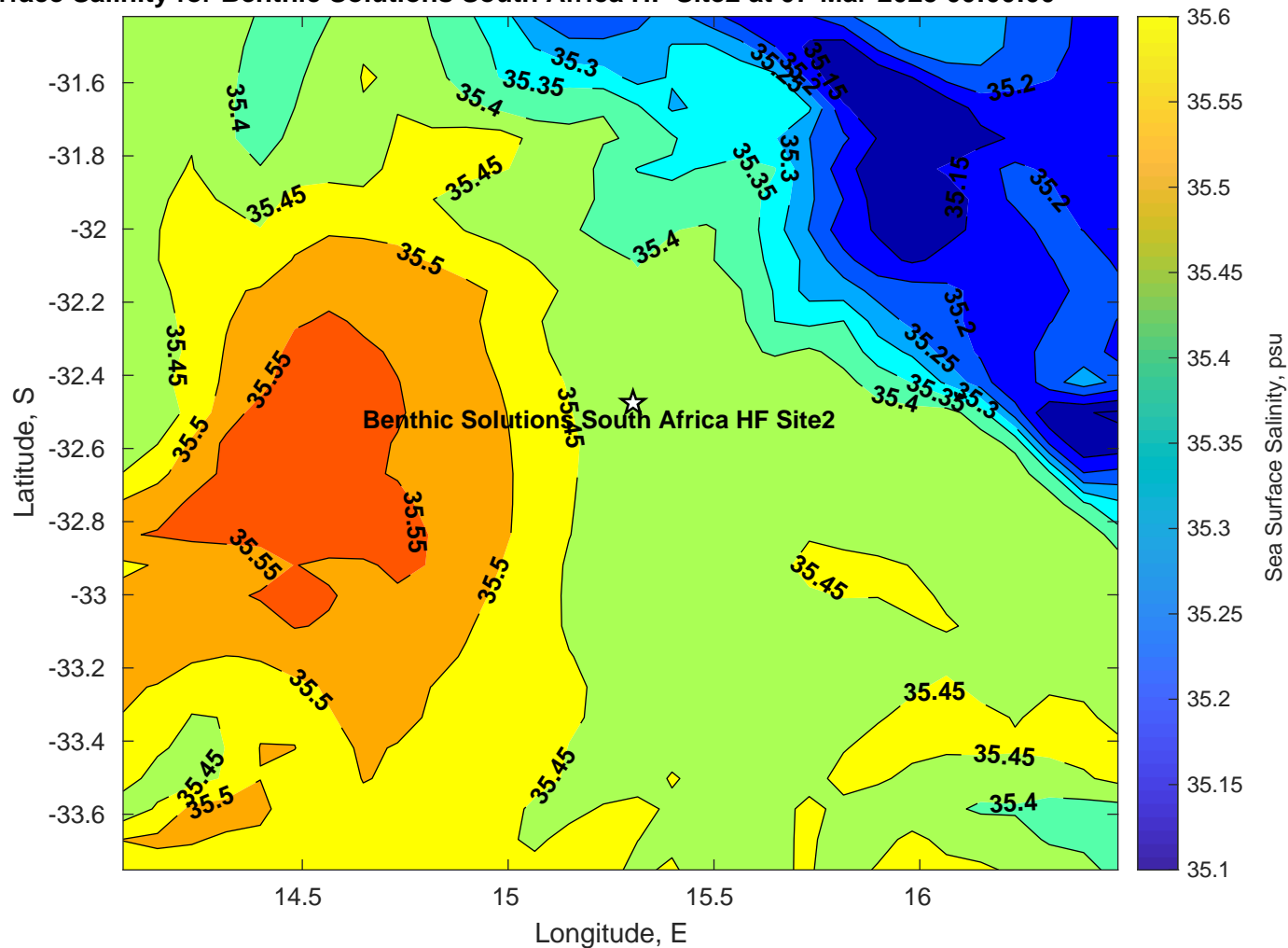
Surface Salinity for Benthic Solutions South Africa HF Site2 at 07-Mar-2025 00:00:00
