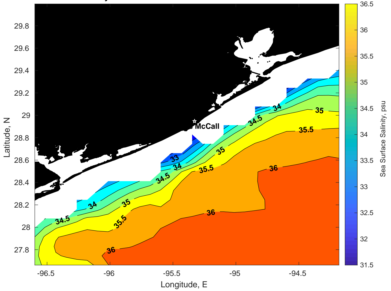
Surface Salinity for Brooks McCall at 07-Mar-2025 00:00:00
