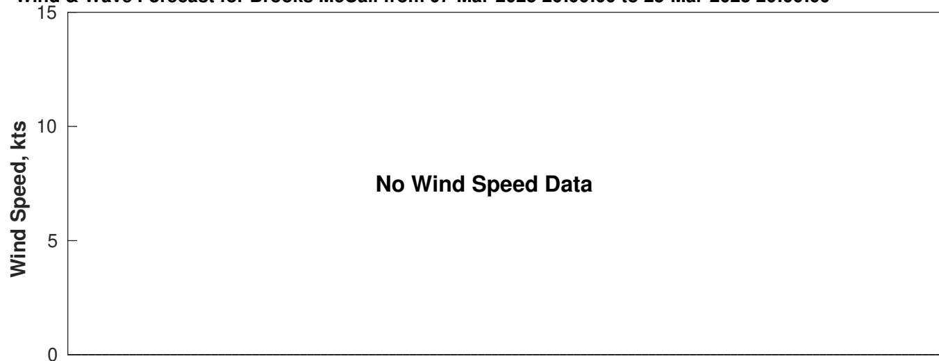
Wind & Wave Forecast for Brooks McCall from 07-Mar-2025 20:00:00 to 23-Mar-2025 20:00:00
