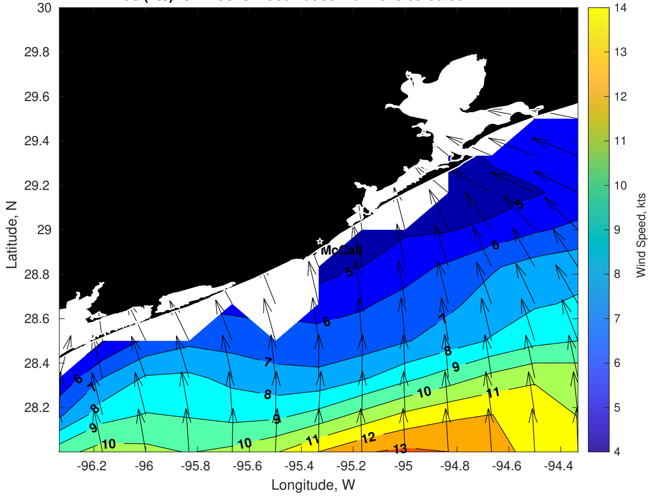
Winds (kts) for Brooks McCall at 08-Mar-2025 09:00:00
