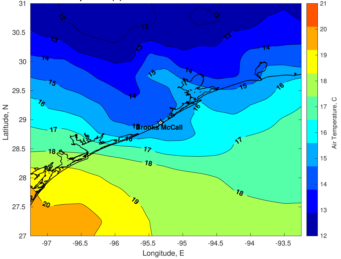
Air Temperature (C) for Brooks McCall at 08-Mar-2025
