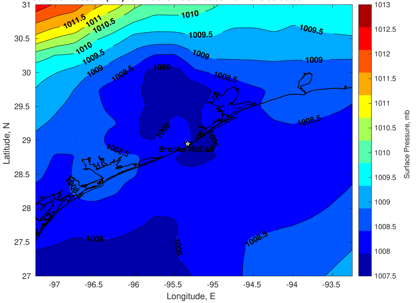
Surface Pressure (mb) for Brooks McCall at 09-Mar-2025 00:00:00
