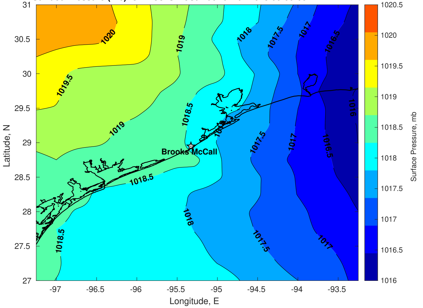
Surface Pressure (mb) for Brooks McCall at 10-Mar-2025 00:00:00
