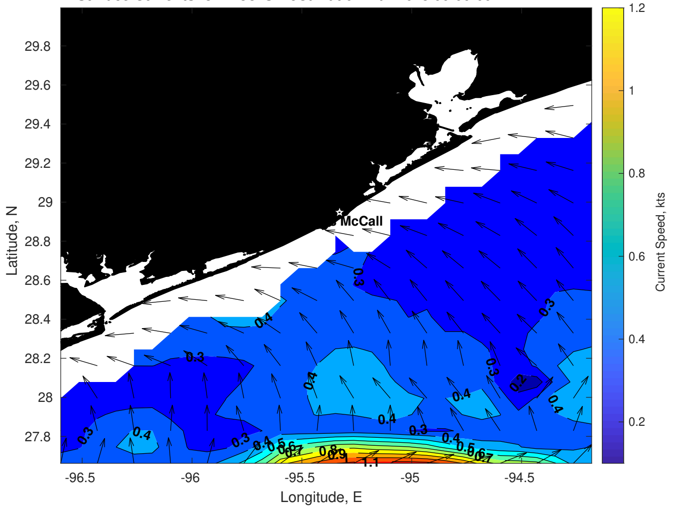
Surface Currents for Brooks McCall at 07-Mar-2025 00:00:00
