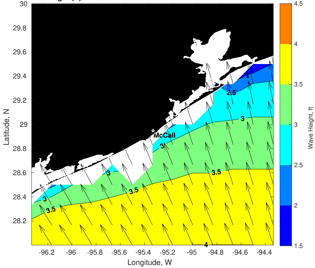
Wave Height (ft) for Brooks McCall at 08-Mar-2025 09:00:00
