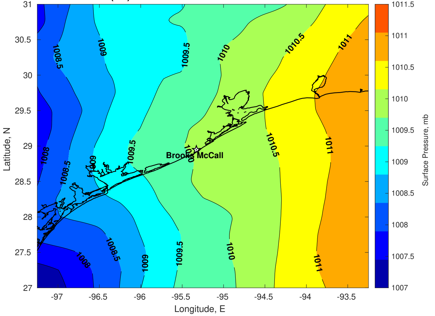
Surface Pressure (mb) for Brooks McCall at 08-Mar-2025 00:00:00
