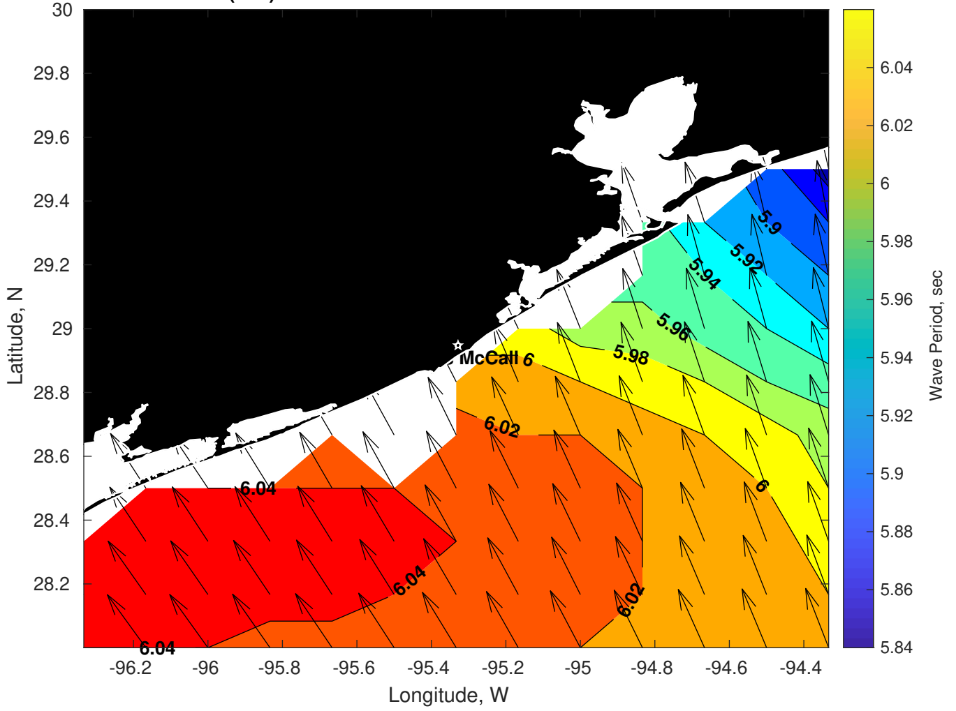
Wave Period (sec) for Brooks McCall at 08-Mar-2025 09:00:00
