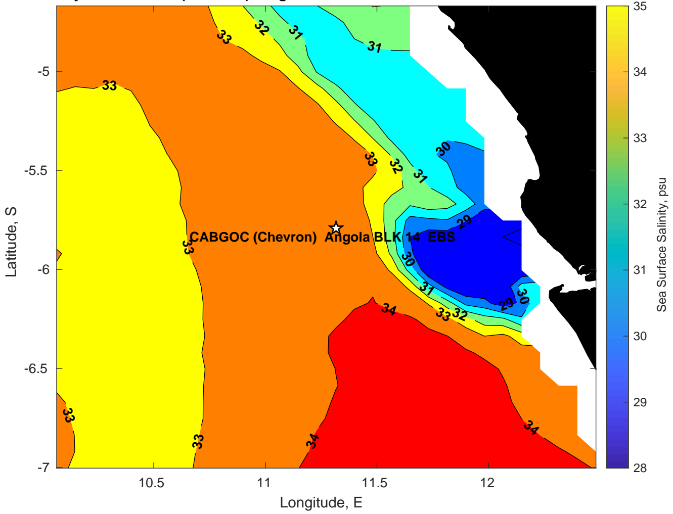
Surface Salinity for CABGOC (Chevron) Angola BLK 14 EBS at 07-Mar-2025 00:00:00
