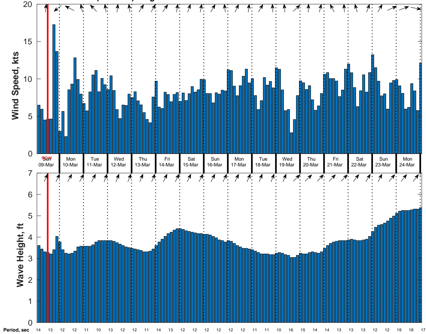
Wind & Wave Forecast for CABGOC (Chevron) Angola BLK 14 EBS from 08-Mar-2025 02:00:00 to 24-Mar-2025 02:00:00
