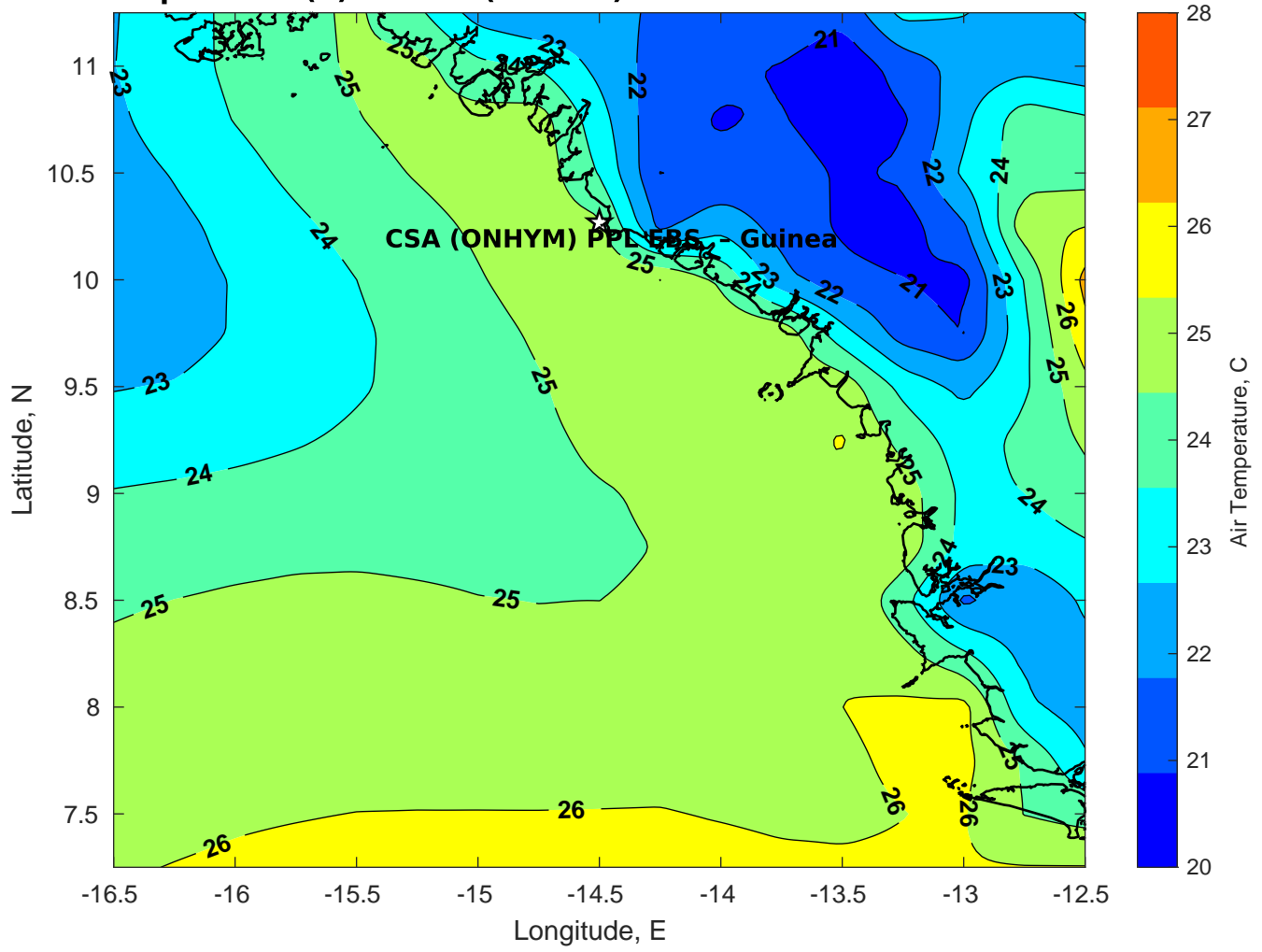
Air Temperature (C) for CSA (ONHYM) PPL EBS - Guinea at 08-Mar-2025
