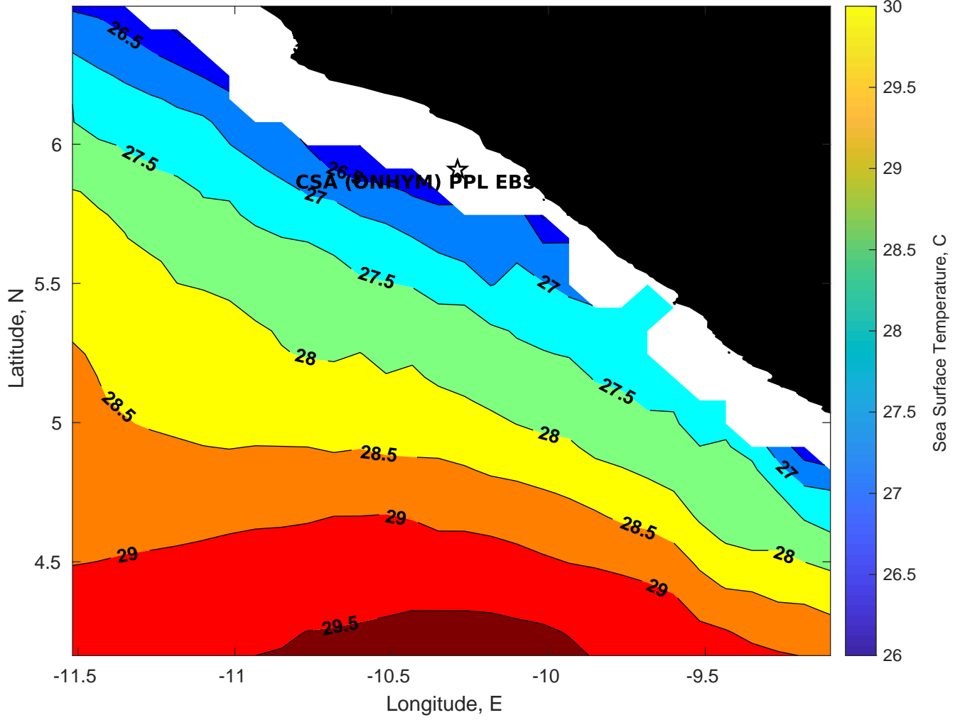
SST for CSA (ONHYM) PPL EBS - Liberia at 07-Mar-2025 00:00:00
