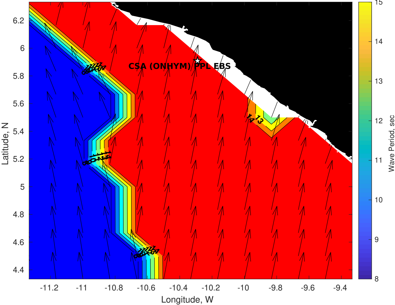
Wave Period (sec) for CSA (ONHYM) PPL EBS - Liberia at 08-Mar-2025 09:00:00
