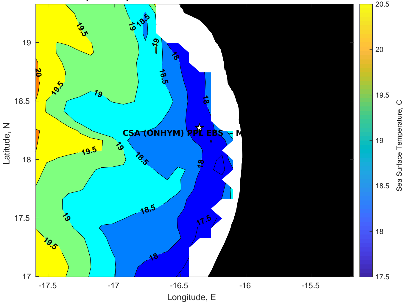
SST for CSA (ONHYM) PPL EBS - Mauritania at 07-Mar-2025 00:00:00
