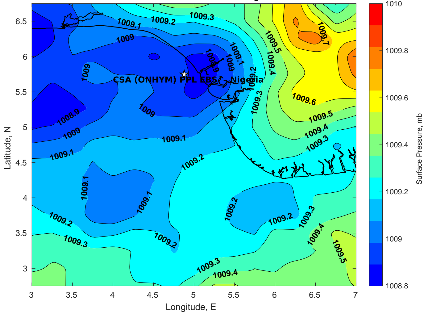
Surface Pressure (mb) for CSA (ONHYM) PPL EBS - Nigeria at 08-Mar-2025 06:00:00
