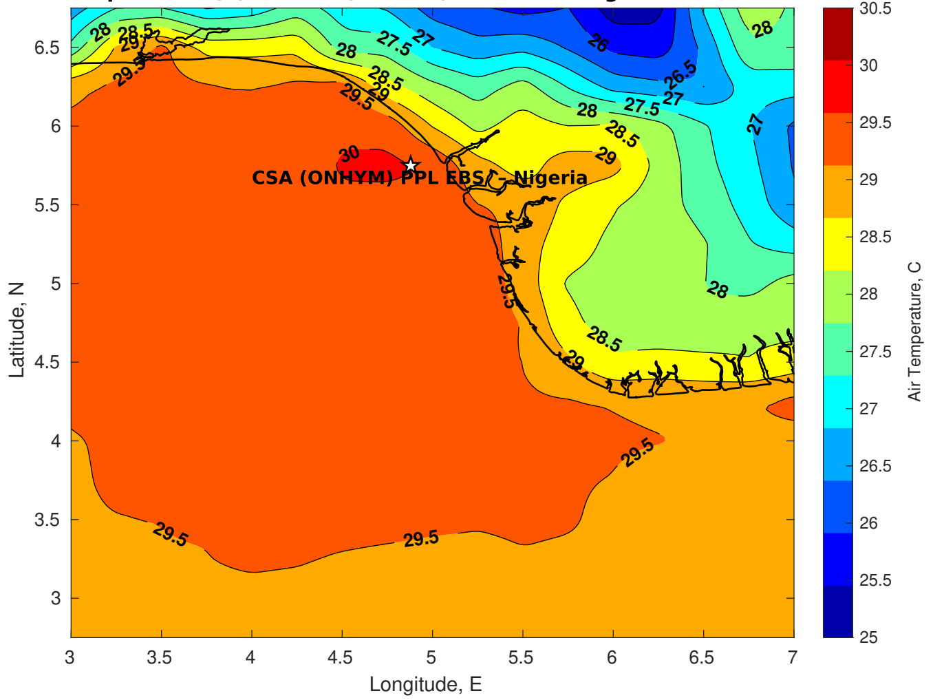
Air Temperature (C) for CSA (ONHYM) PPL EBS - Nigeria at 08-Mar-2025
