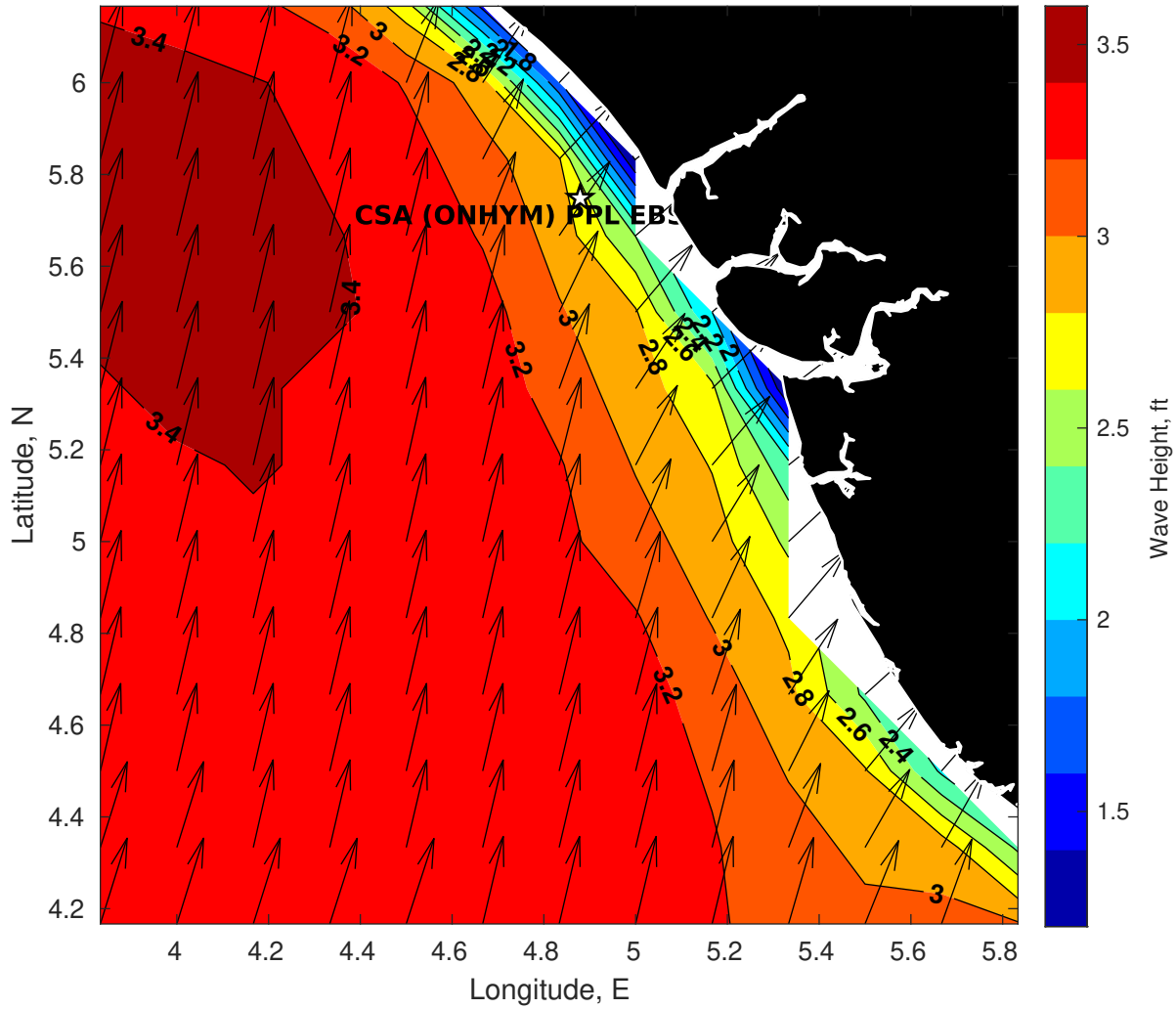
Wave Height (ft) for CSA (ONHYM) PPL EBS - Nigeria at 08-Mar-2025 09:00:00
