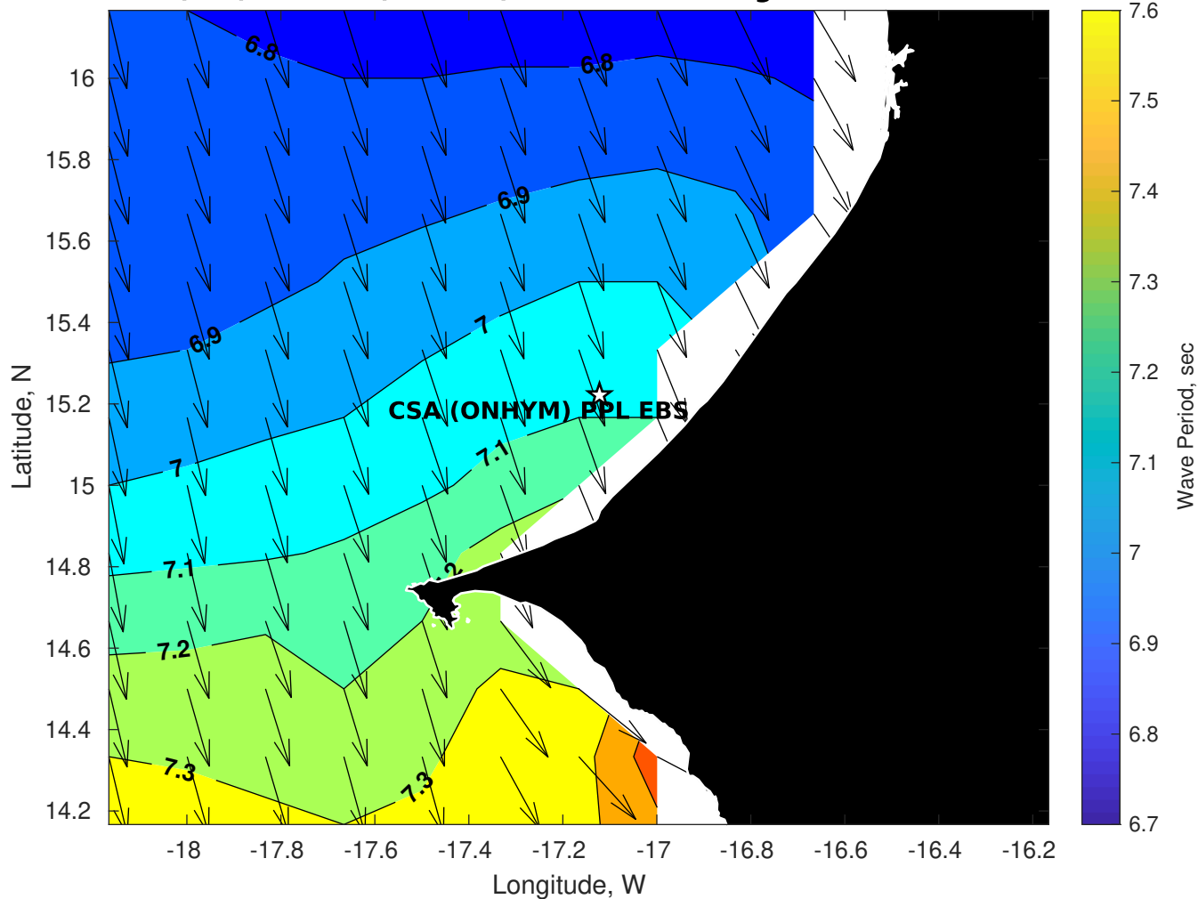
Wave Period (sec) for CSA (ONHYM) PPL EBS - Senegal at 08-Mar-2025 09:00:00
