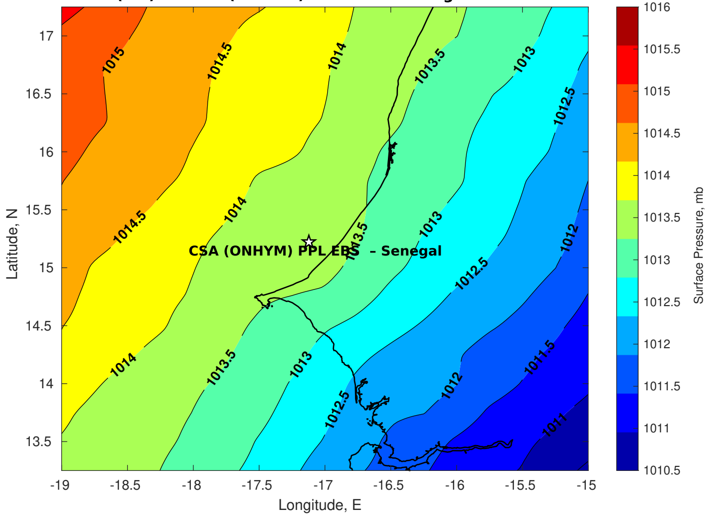
Surface Pressure (mb) for CSA (ONHYM) PPL EBS - Senegal at 08-Mar-2025 00:00:00
