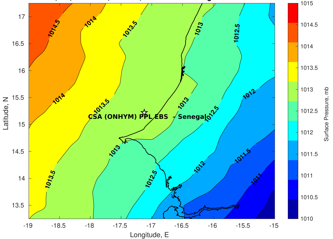
Surface Pressure (mb) for CSA (ONHYM) PPL EBS - Senegal at 09-Mar-2025 00:00:00
