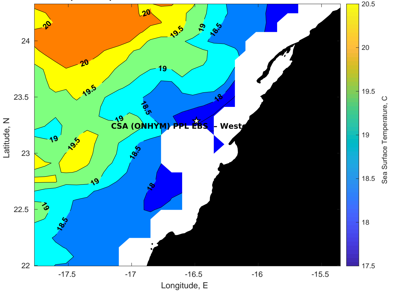
SST for CSA (ONHYM) PPL EBS - Western Sahara at 07-Mar-2025 00:00:00
