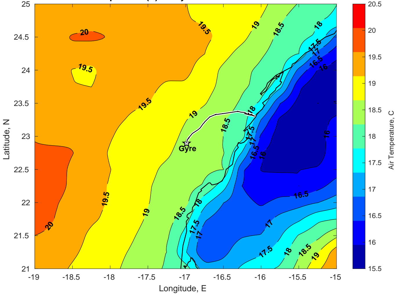
Air Temperature (C) for Gyre at 08-Mar-2025
