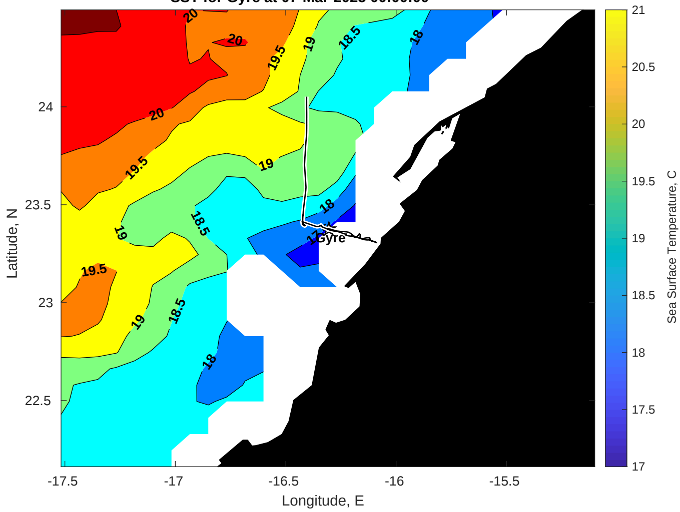
SST for Gyre at 07-Mar-2025 00:00:00
