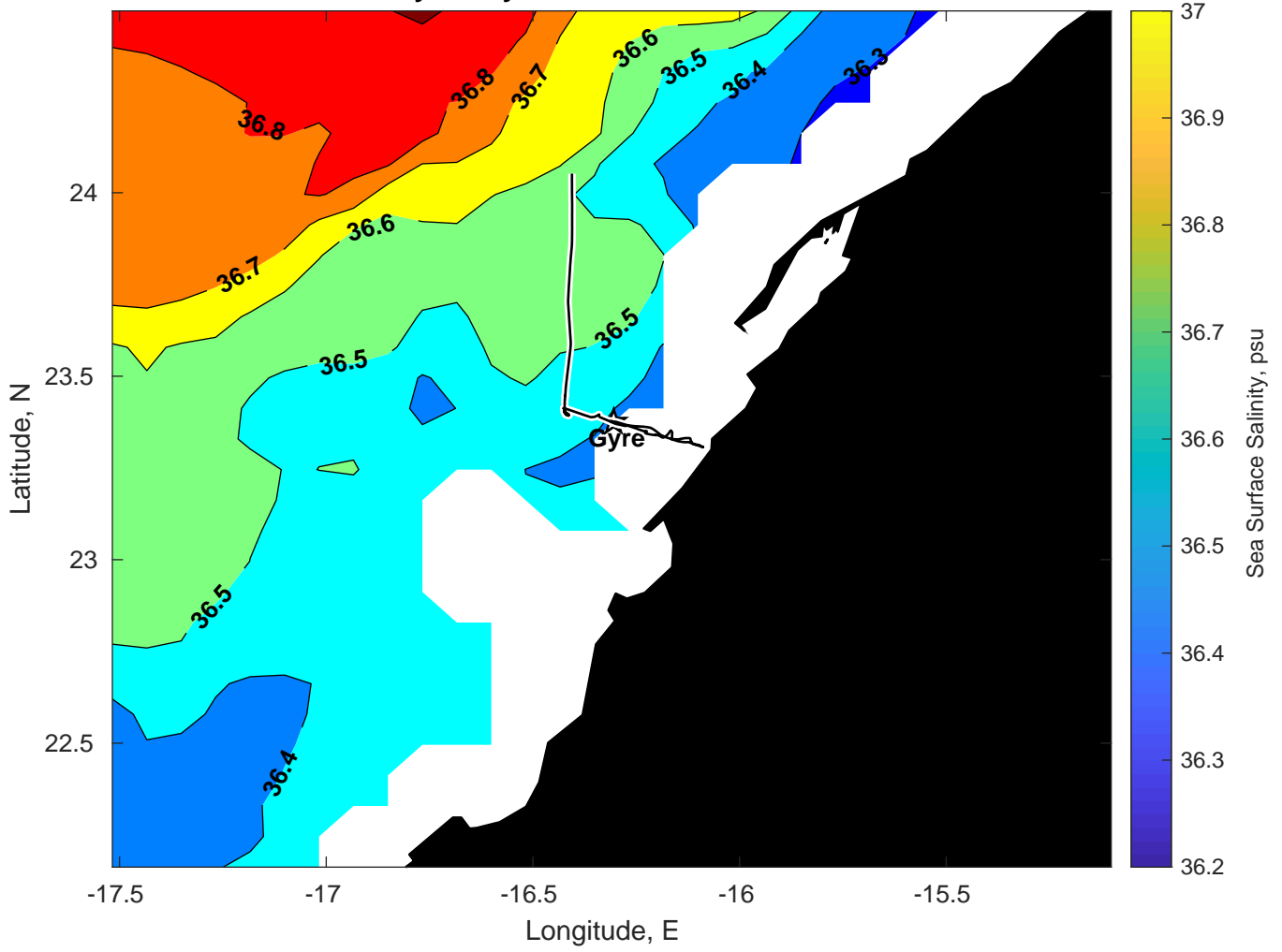
Surface Salinity for Gyre at 07-Mar-2025 00:00:00
