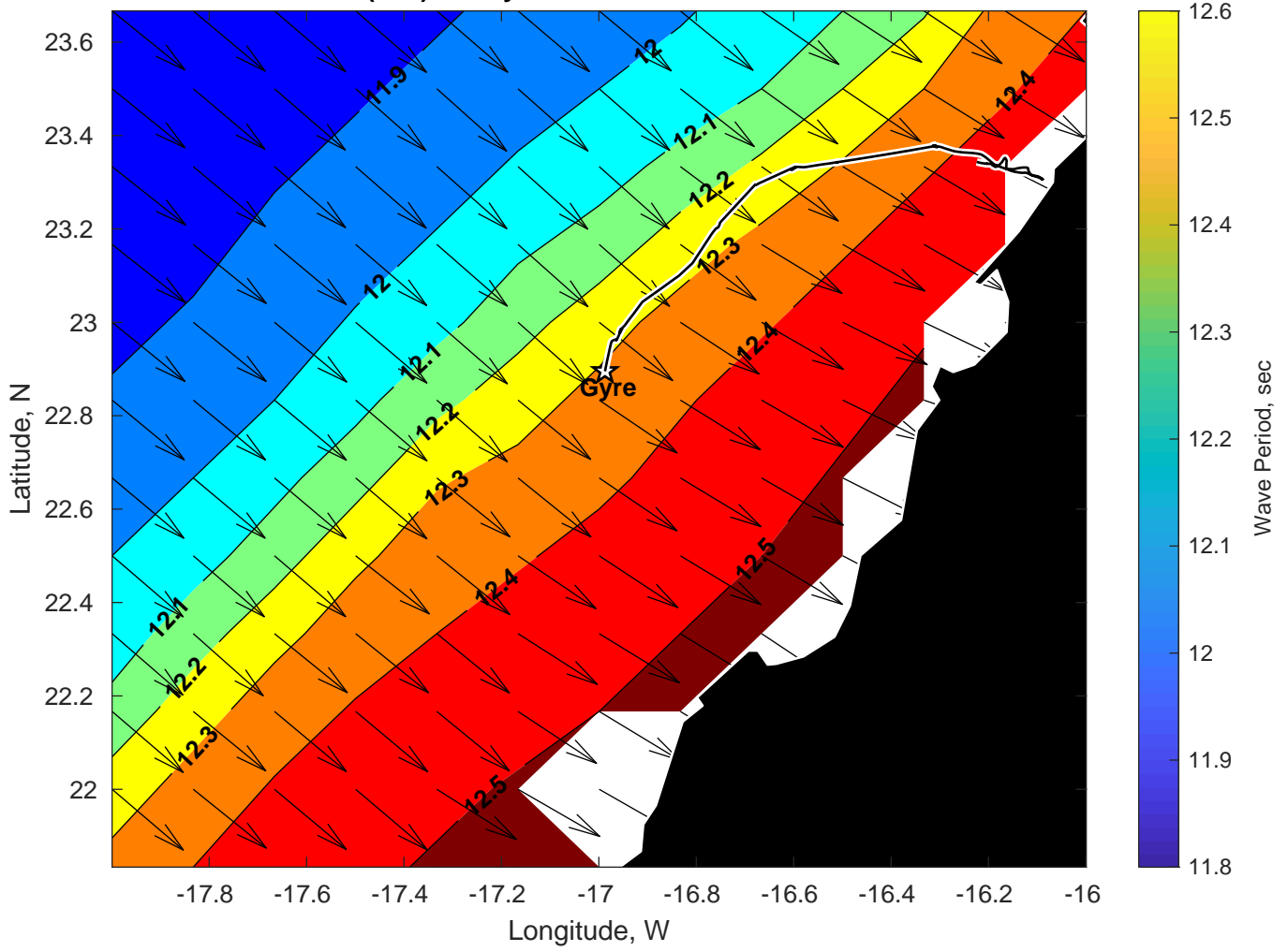
Wave Period (sec) for Gyre at 08-Mar-2025 09:00:00
