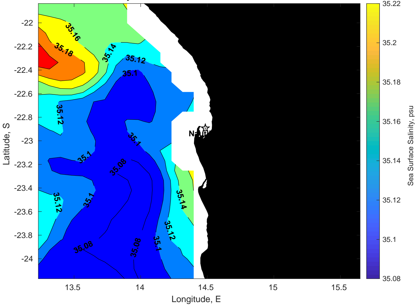
Surface Salinity for Nautilus at 07-Mar-2025 00:00:00
