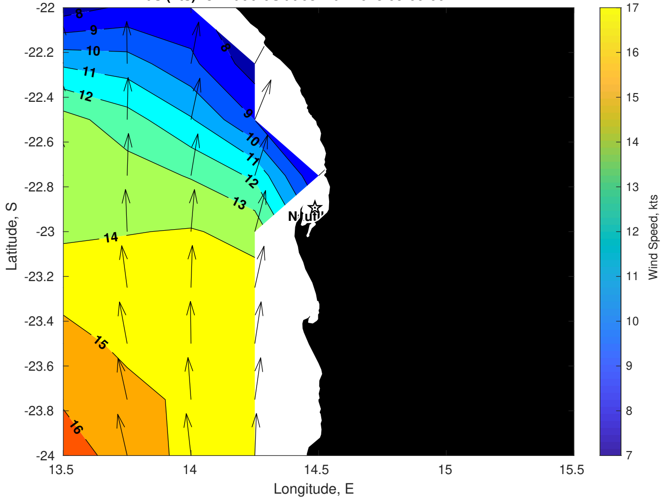
Winds (kts) for Nautilus at 08-Mar-2025 09:00:00
