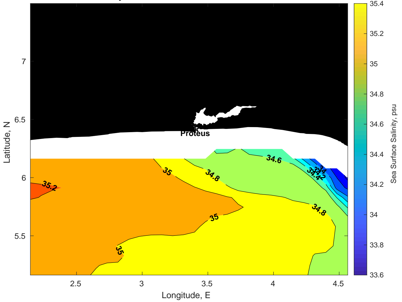
Surface Salinity for Proteus at 07-Mar-2025 00:00:00
