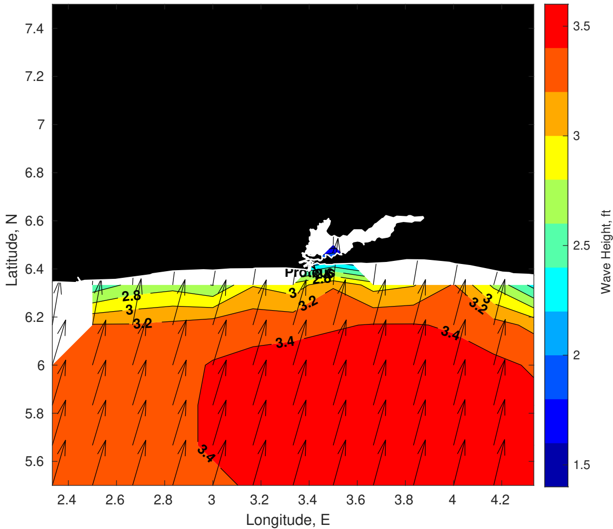
Wave Height (ft) for Proteus at 08-Mar-2025 09:00:00
