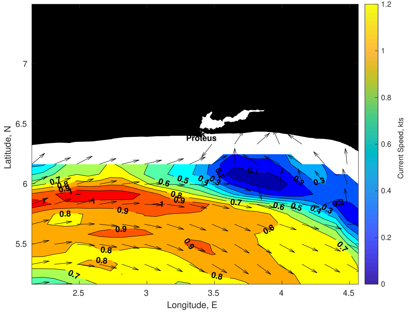
Surface Currents for Proteus at 07-Mar-2025 00:00:00
