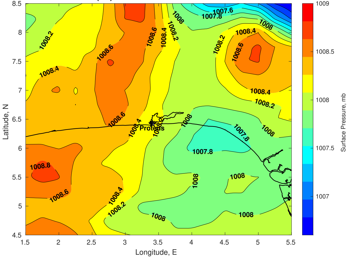
Surface Pressure (mb) for Proteus at 09-Mar-2025 00:00:00
