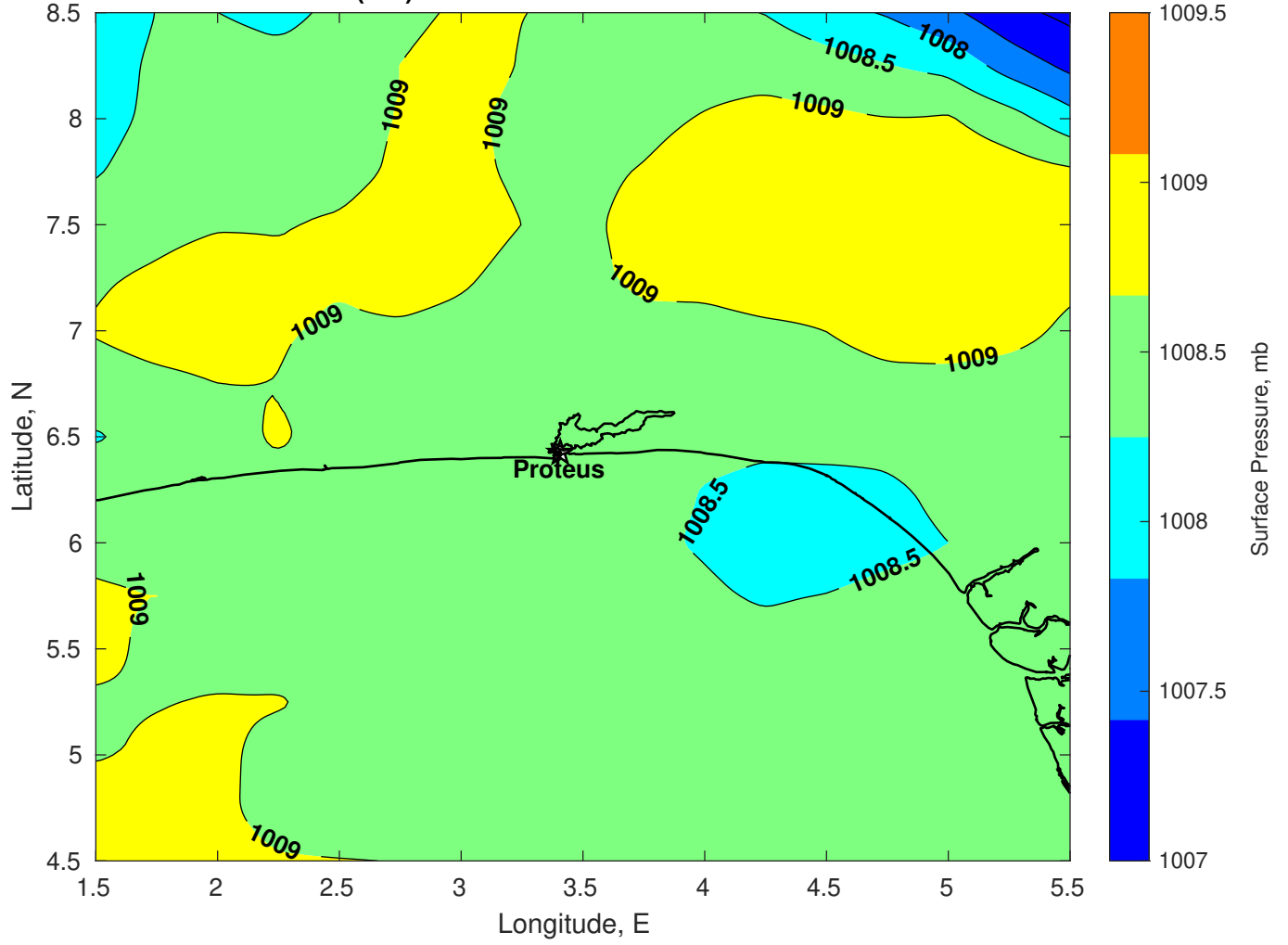
Surface Pressure (mb) for Proteus at 10-Mar-2025 00:00:00
