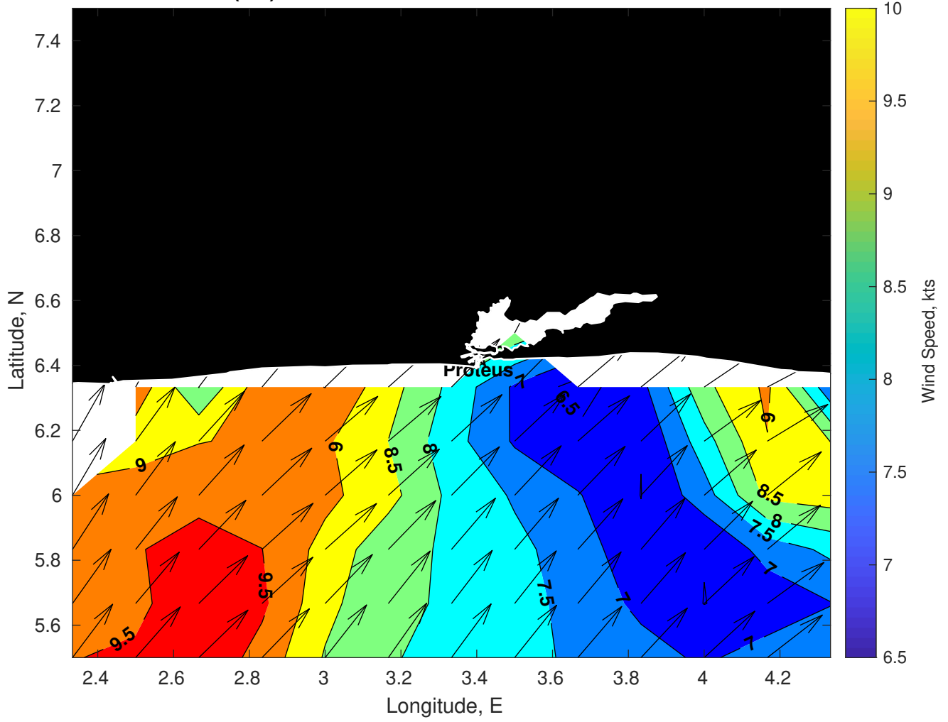
Winds (kts) for Proteus at 08-Mar-2025 09:00:00
