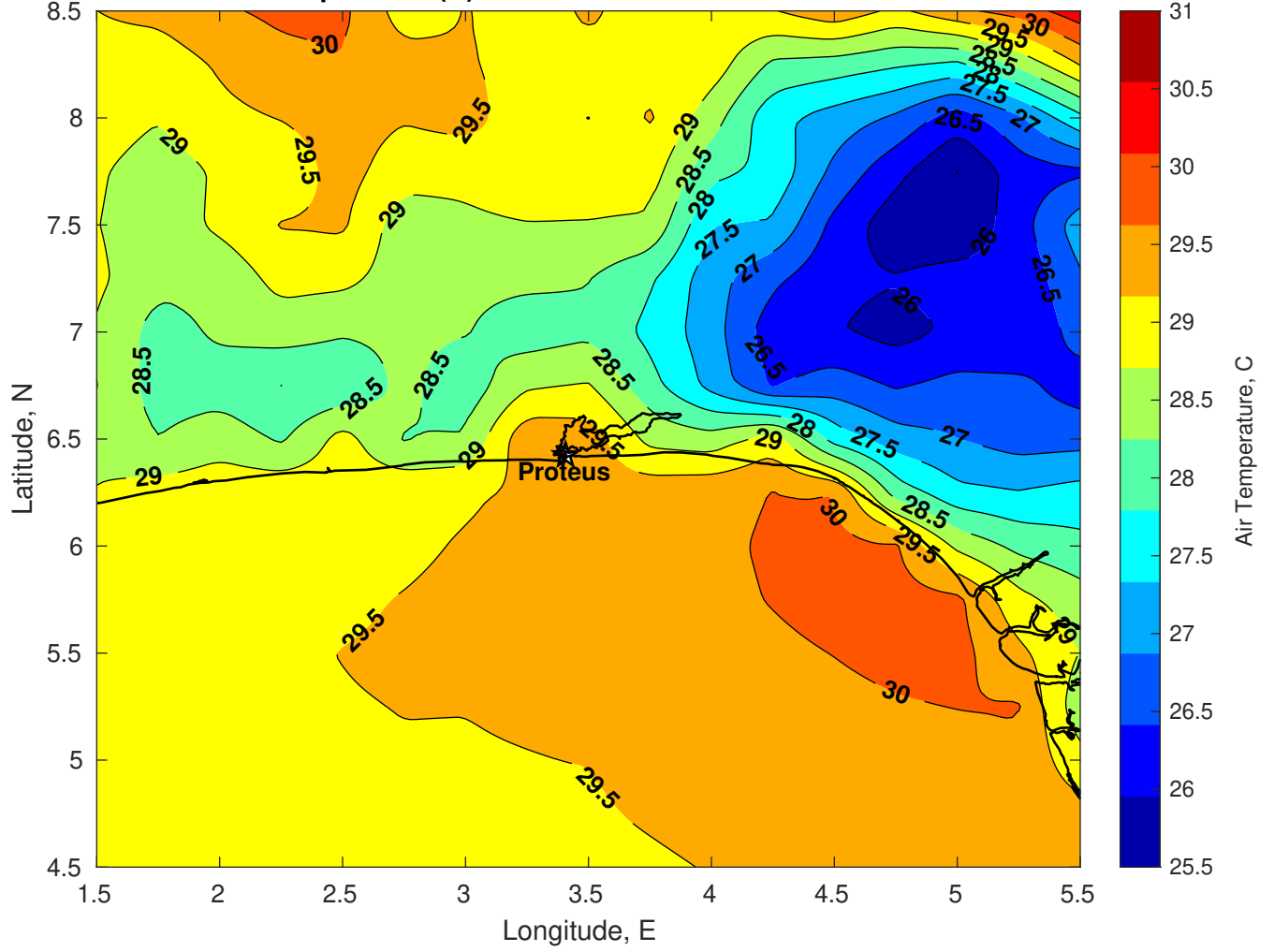
Air Temperature (C) for Proteus at 08-Mar-2025
