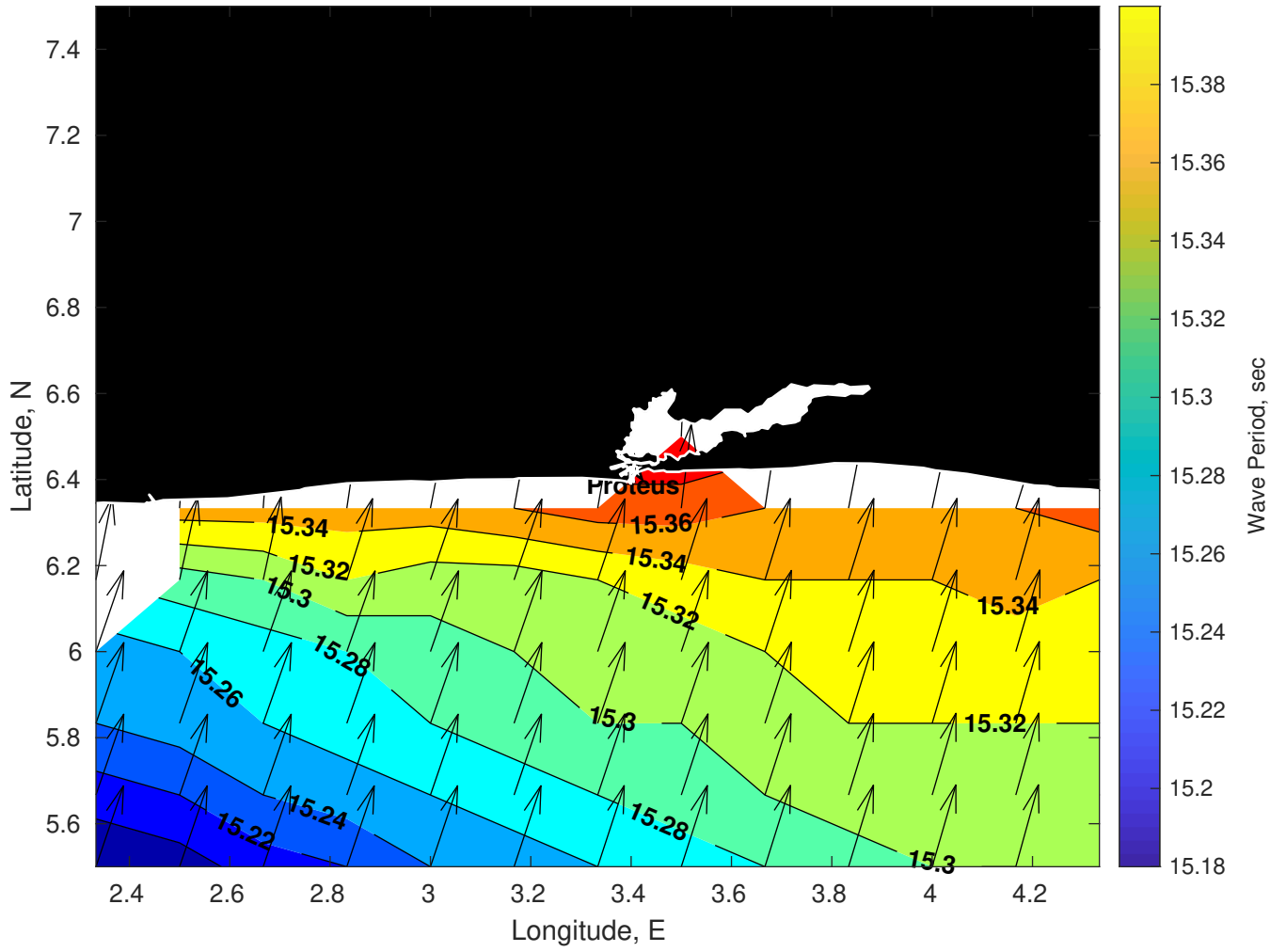
Wave Period (sec) for Proteus at 08-Mar-2025 09:00:00
