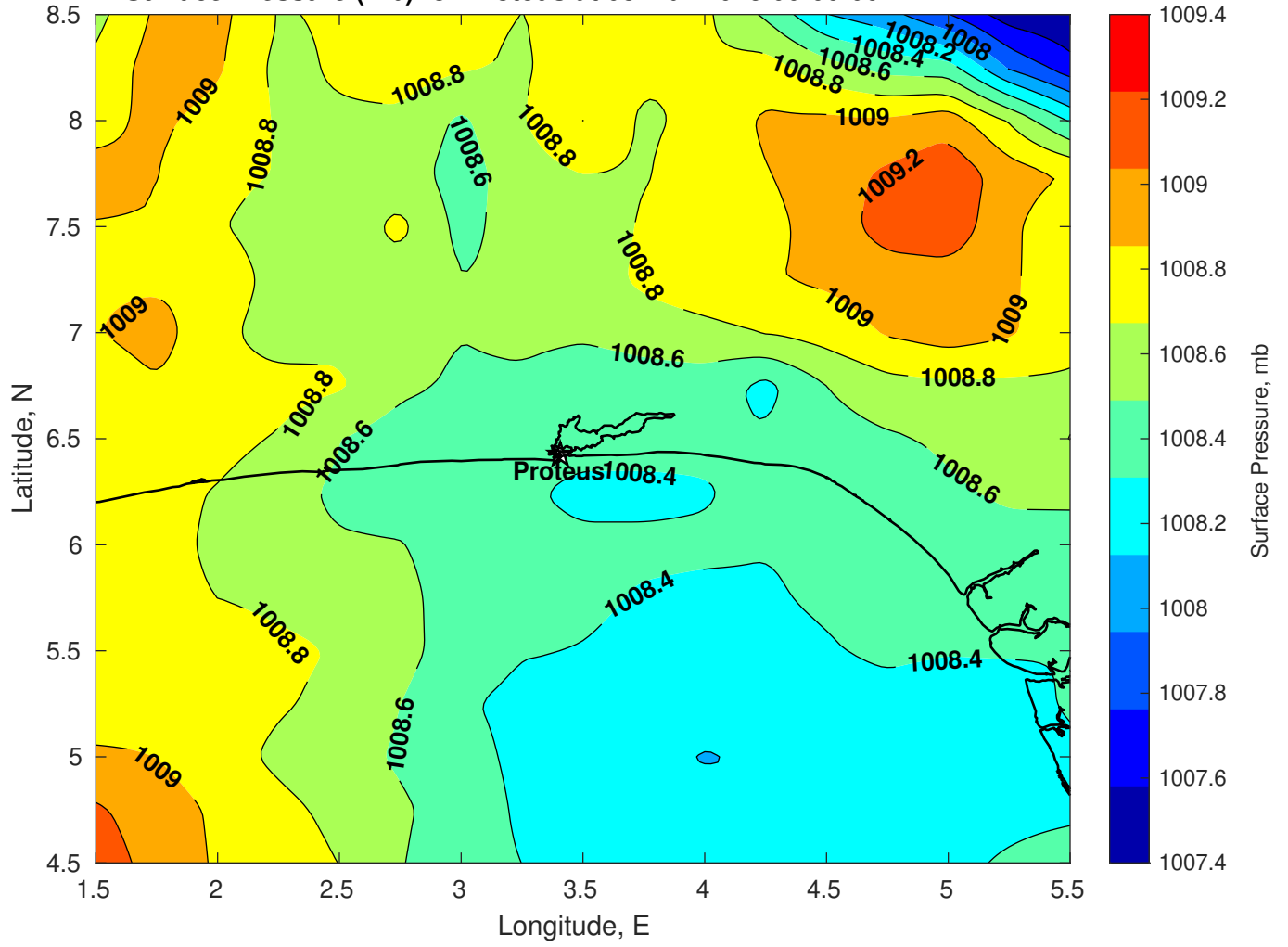
Surface Pressure (mb) for Proteus at 08-Mar-2025 00:00:00
