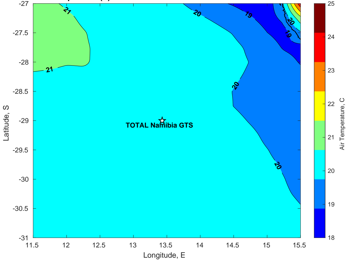
Air Temperature (C) for TOTAL Namibia GTS at 08-Mar-2025
