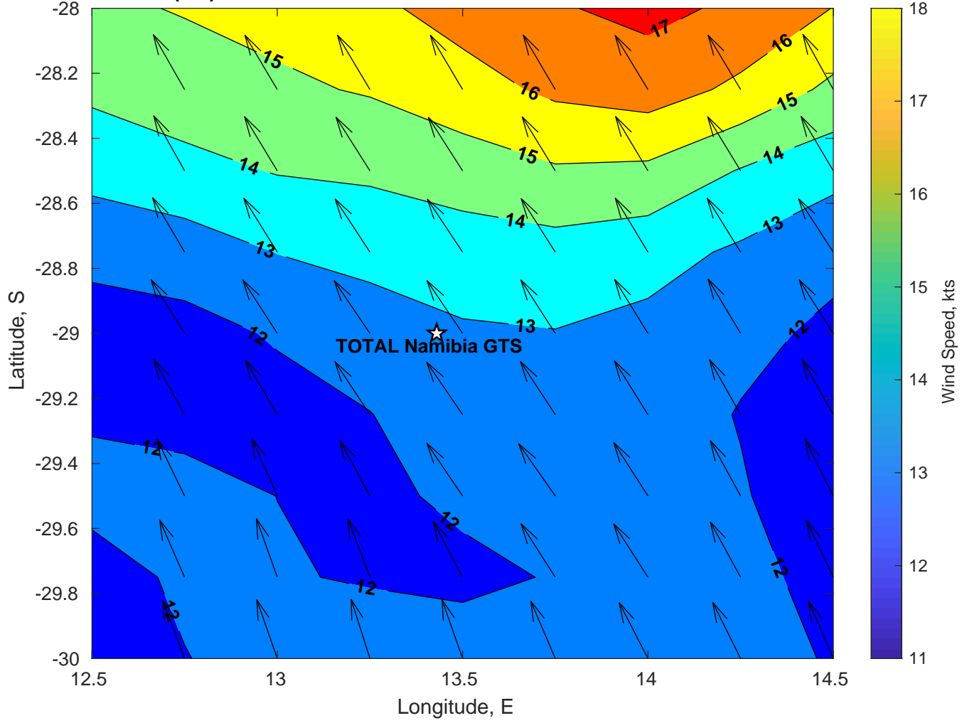
Winds (kts) for TOTAL Namibia GTS at 08-Mar-2025 09:00:00
