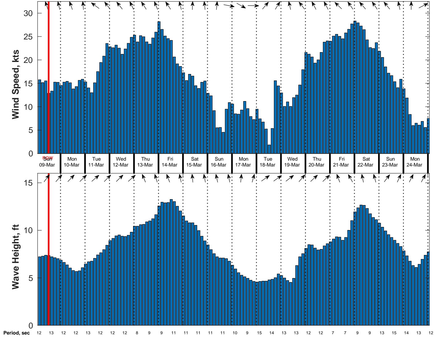
Wind & Wave Forecast for TOTAL Namibia GTS from 08-Mar-2025 02:00:00 to 24-Mar-2025 02:00:00
