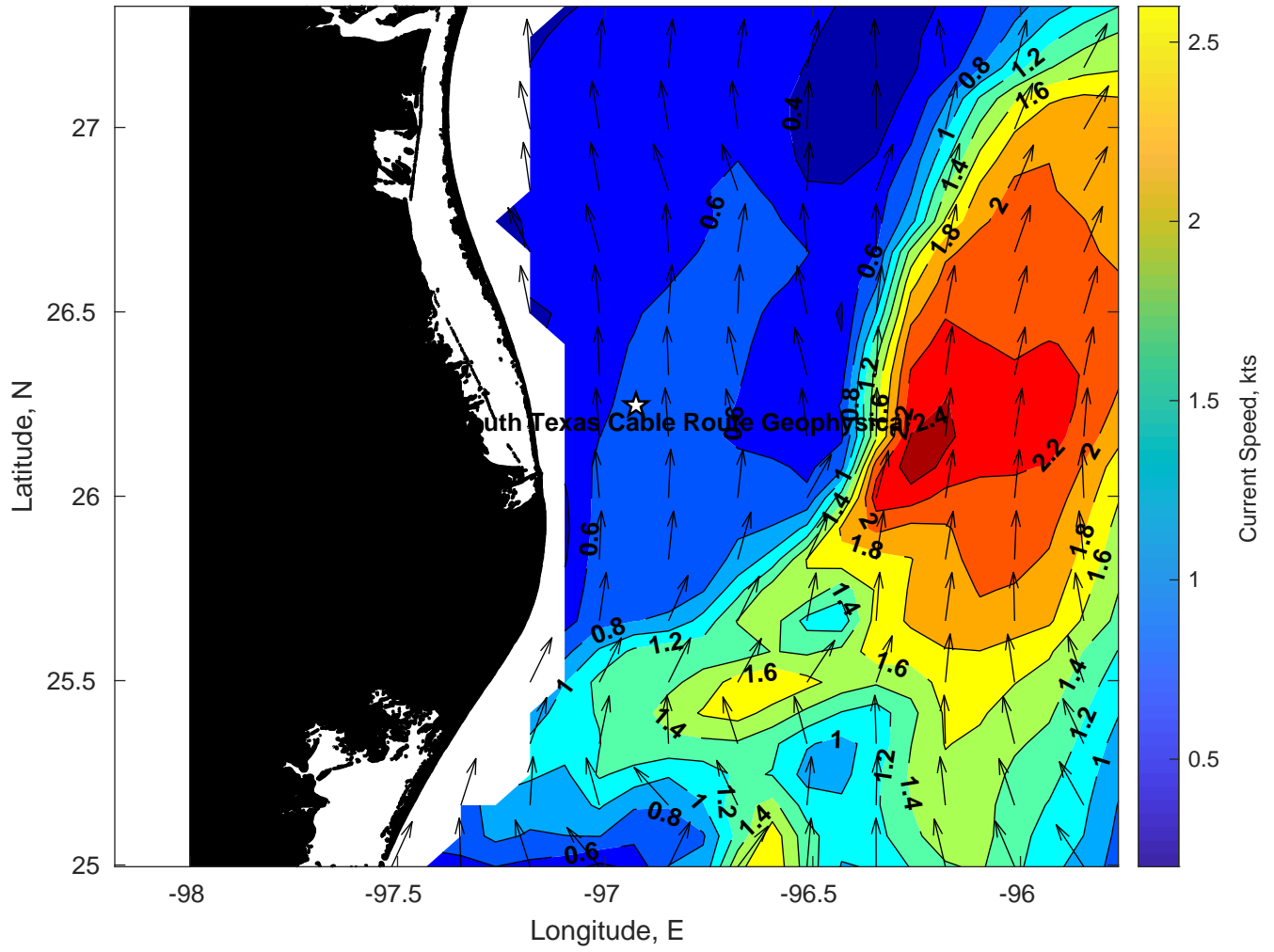
Surface Currents for Tampnet P2378 South Texas Cable Route Geophysical at 07-Mar-2025 00:00:00
