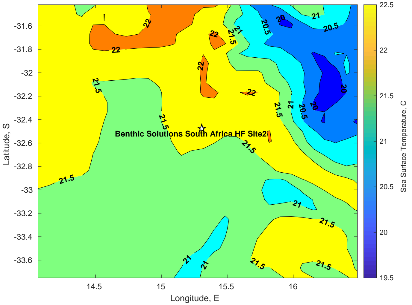
SST for Benthic Solutions South Africa HF Site2 at 08-Mar-2025 00:00:00
