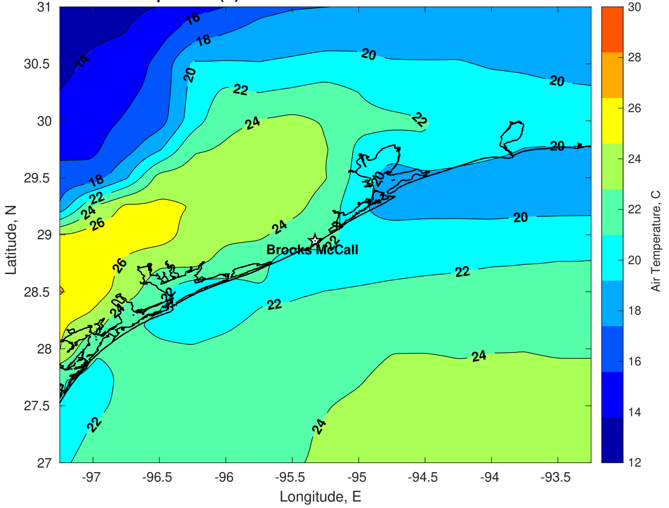
Air Temperature (C) for Brooks McCall at 09-Mar-2025
