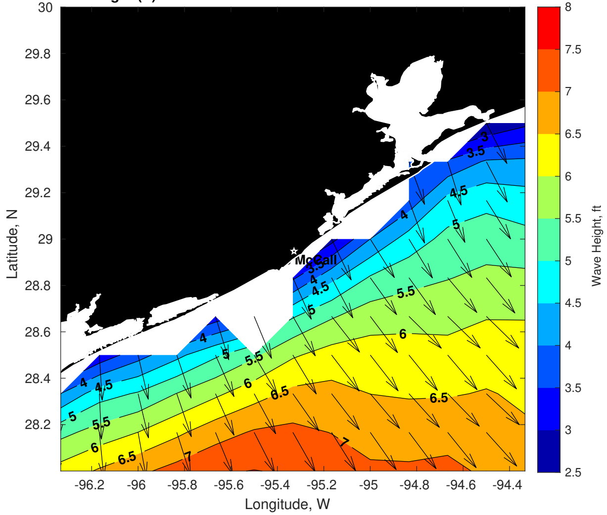
Wave Height (ft) for Brooks McCall at 09-Mar-2025 09:00:00
