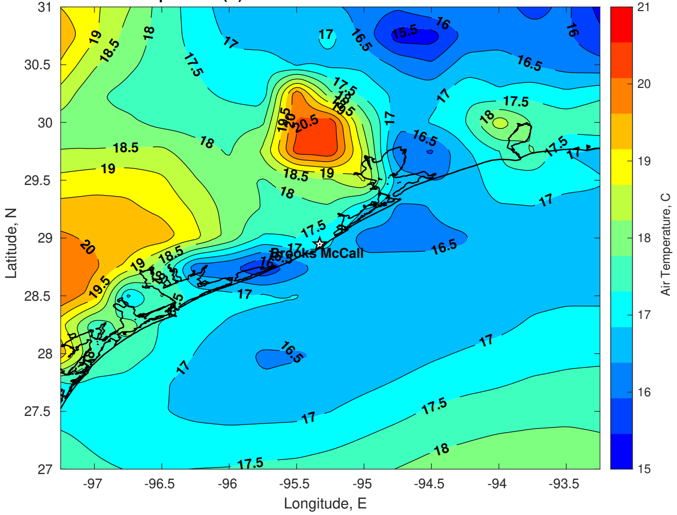
Air Temperature (C) for Brooks McCall at 09-Mar-2025
