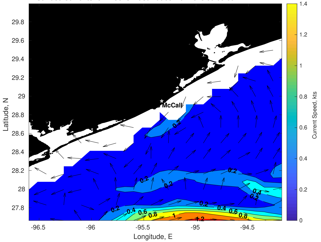
Surface Currents for Brooks McCall at 08-Mar-2025 00:00:00
