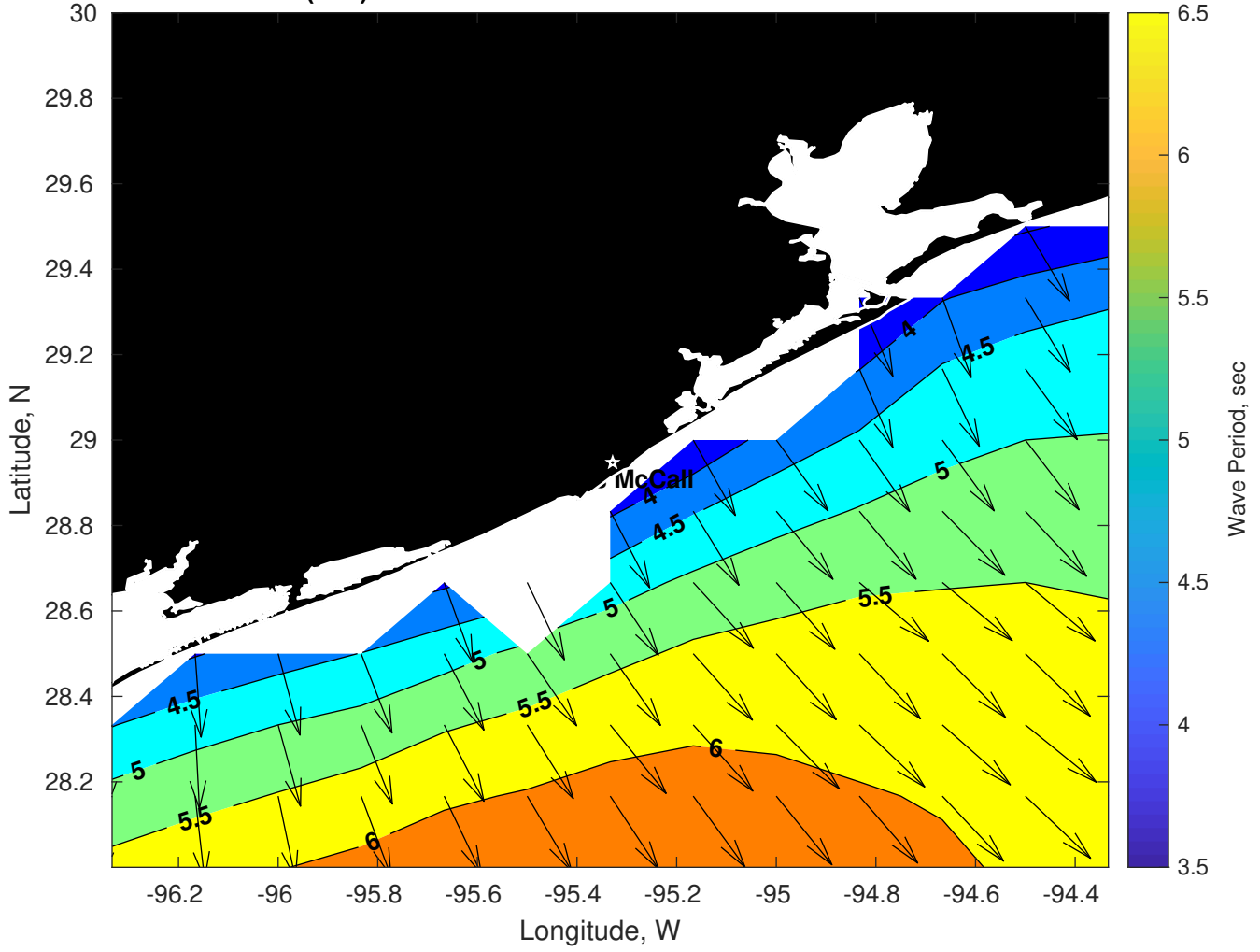
Wave Period (sec) for Brooks McCall at 09-Mar-2025 09:00:00
