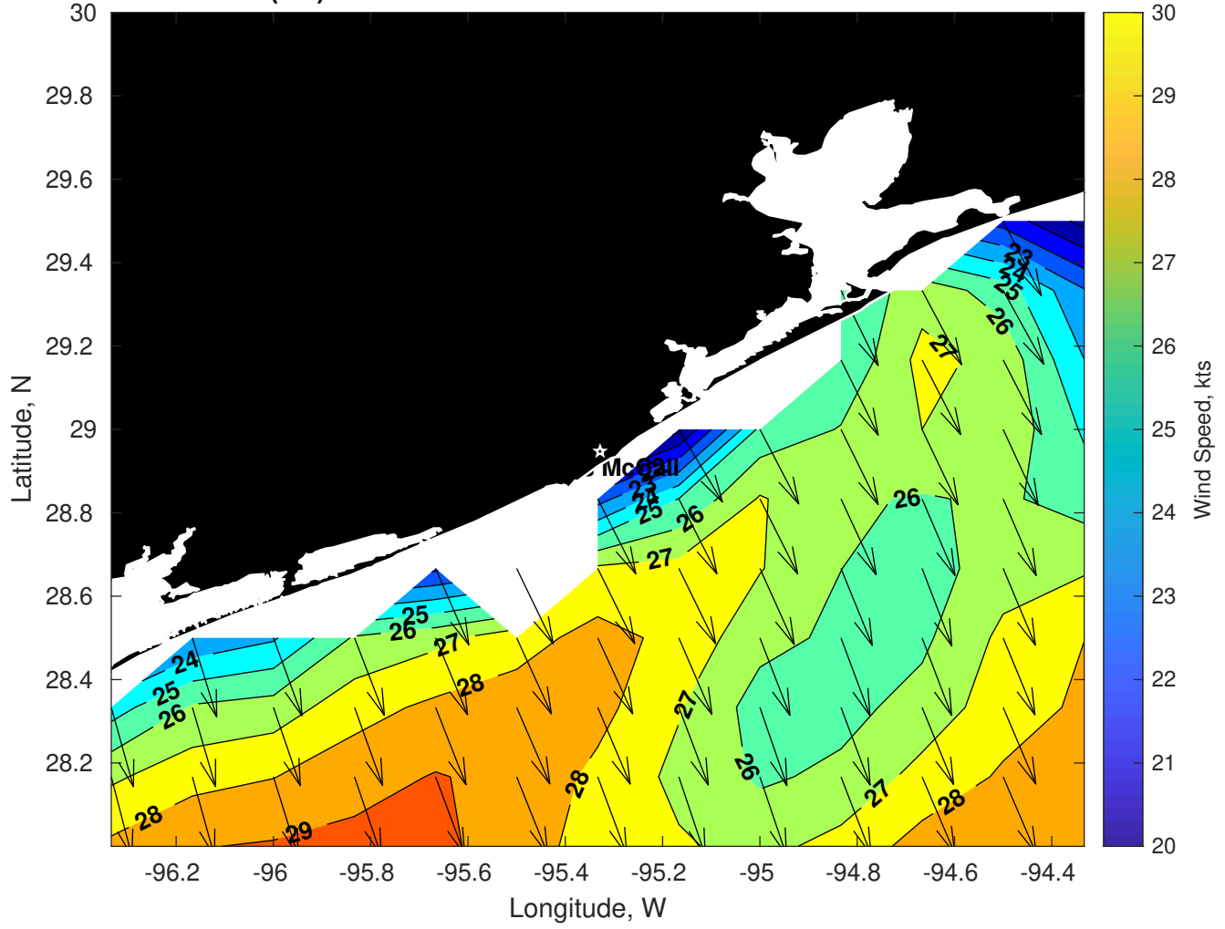
Winds (kts) for Brooks McCall at 09-Mar-2025 09:00:00
