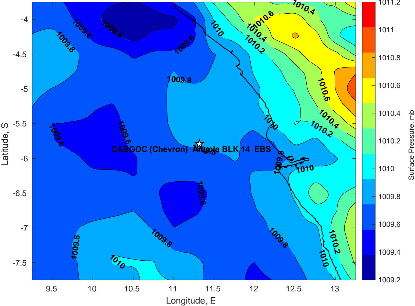
Surface Pressure (mb) for CABGOC (Chevron) Angola BLK 14 EBS at 10-Mar-2025 00:00:00
