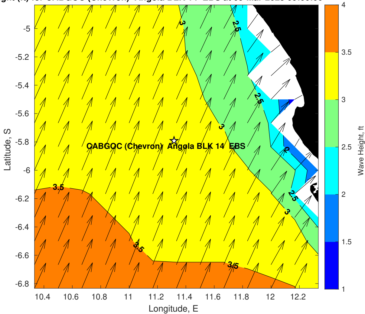
Wave Height (ft) for CABGOC (Chevron) Angola BLK 14 EBS at 09-Mar-2025 09:00:00
