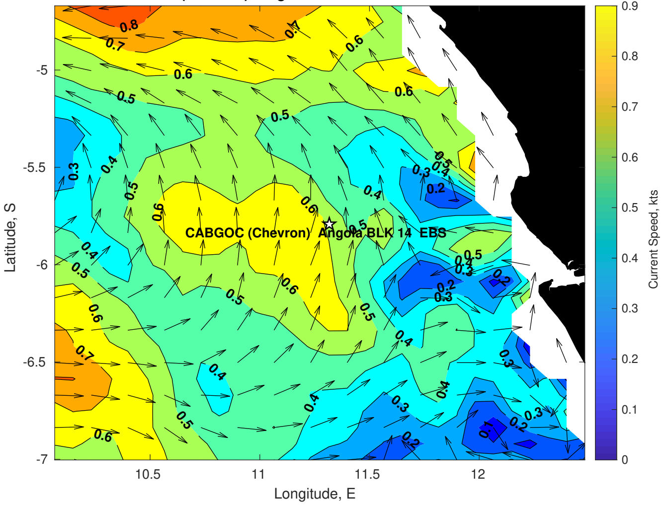
Surface Currents for CABGOC (Chevron) Angola BLK 14 EBS at 08-Mar-2025 00:00:00
