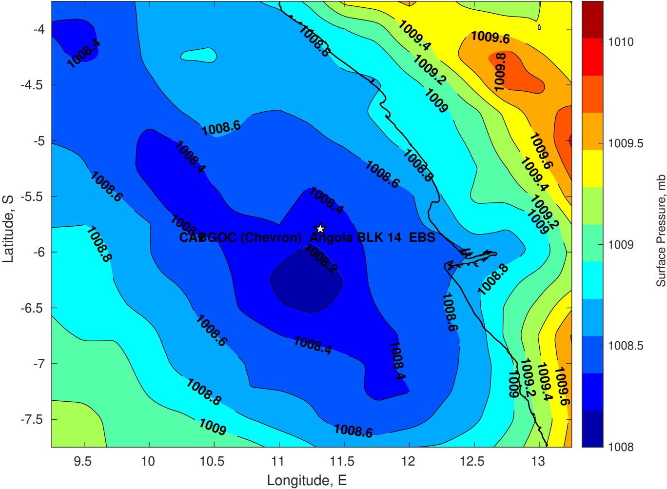
Surface Pressure (mb) for CABGOC (Chevron) Angola BLK 14 EBS at 09-Mar-2025 00:00:00
