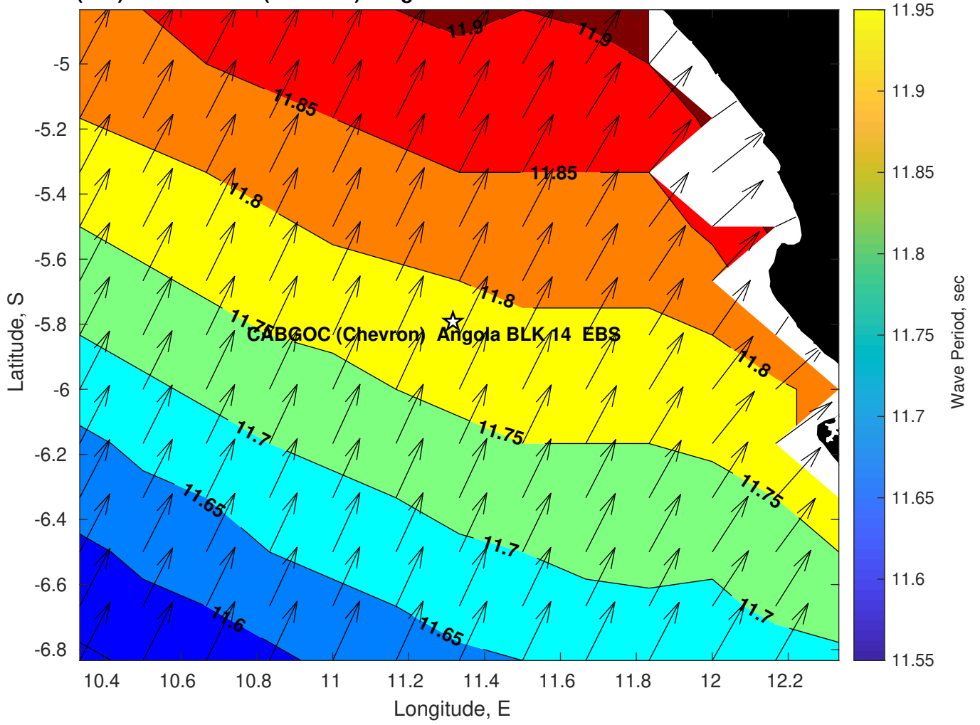
Wave Period (sec) for CABGOC (Chevron) Angola BLK 14 EBS at 09-Mar-2025 09:00:00
