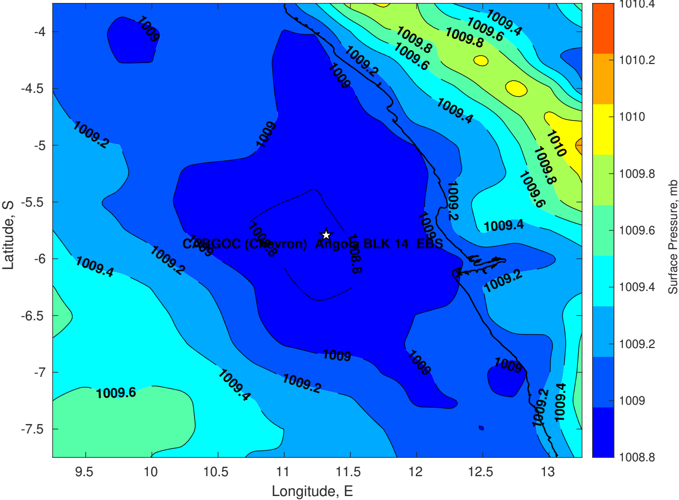
Surface Pressure (mb) for CABGOC (Chevron) Angola BLK 14 EBS at 11-Mar-2025 00:00:00
