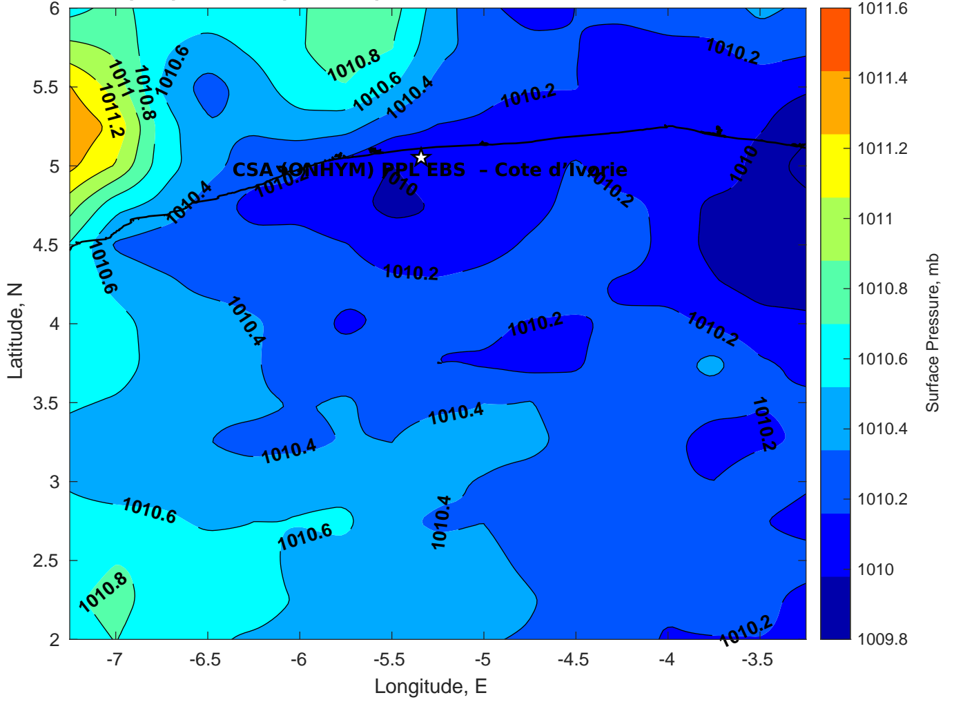
Surface Pressure (mb) for CSA (ONHYM) PPL EBS - Cote d'Ivoire at 09-Mar-2025 00:00:00
