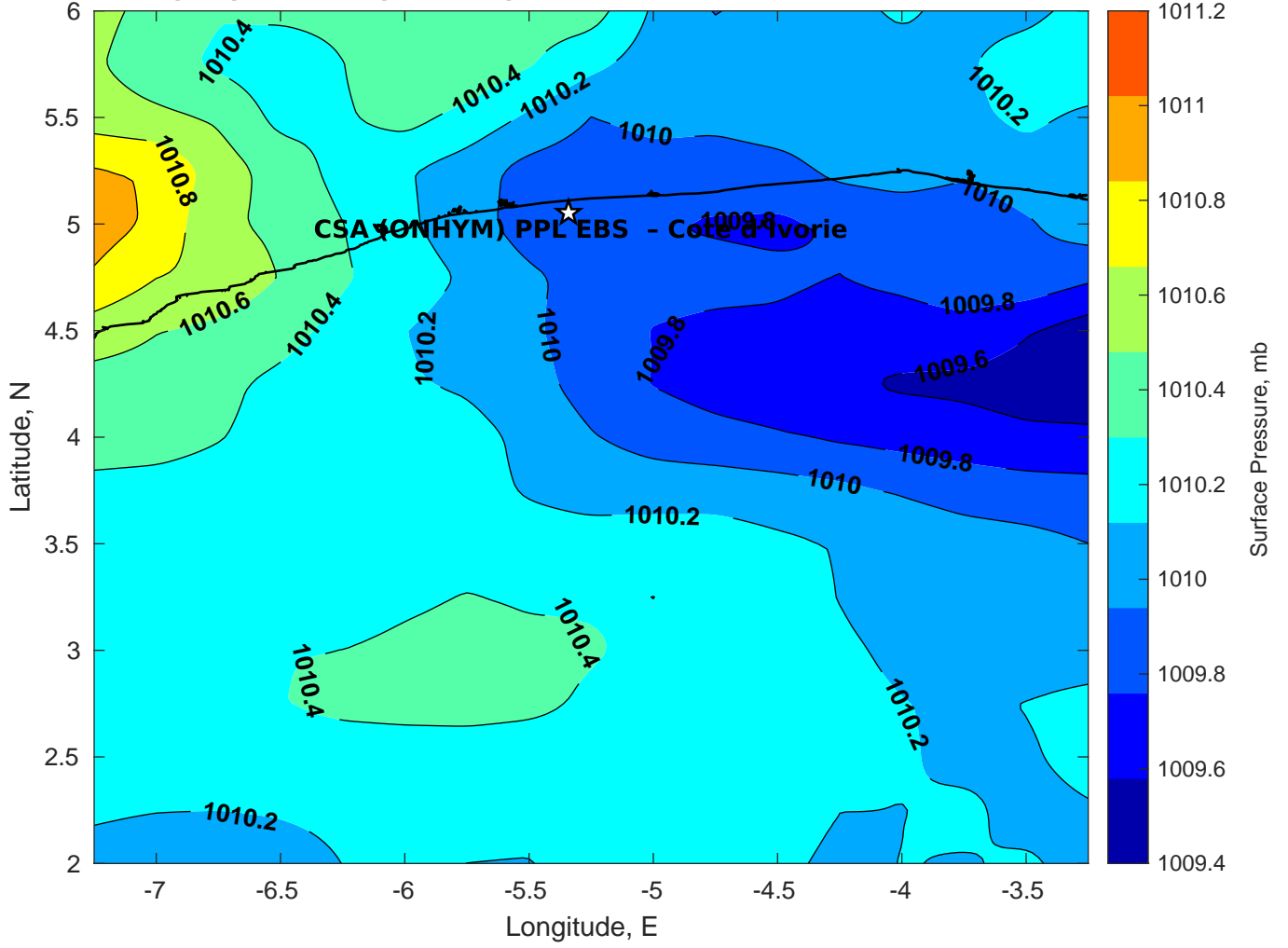
Surface Pressure (mb) for CSA (ONHYM) PPL EBS - Cote d'Ivoire at 10-Mar-2025 00:00:00
