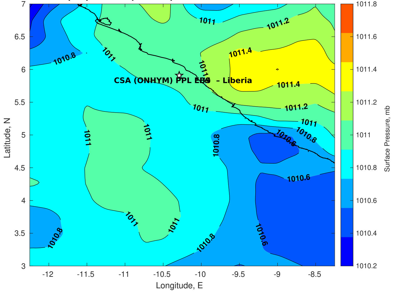
Surface Pressure (mb) for CSA (ONHYM) PPL EBS - Liberia at 10-Mar-2025 00:00:00
