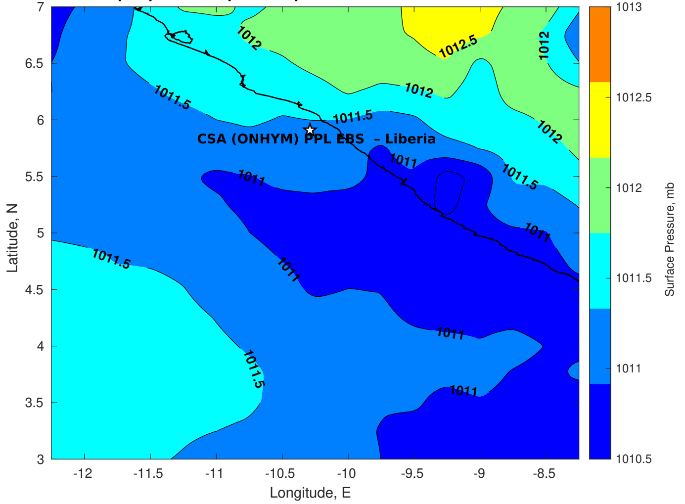
Surface Pressure (mb) for CSA (ONHYM) PPL EBS - Liberia at 09-Mar-2025 00:00:00
