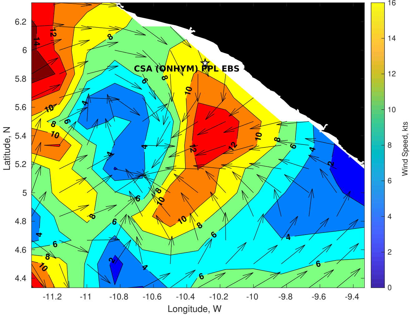
Winds (kts) for CSA (ONHYM) PPL EBS - Liberia at 09-Mar-2025 09:00:00
