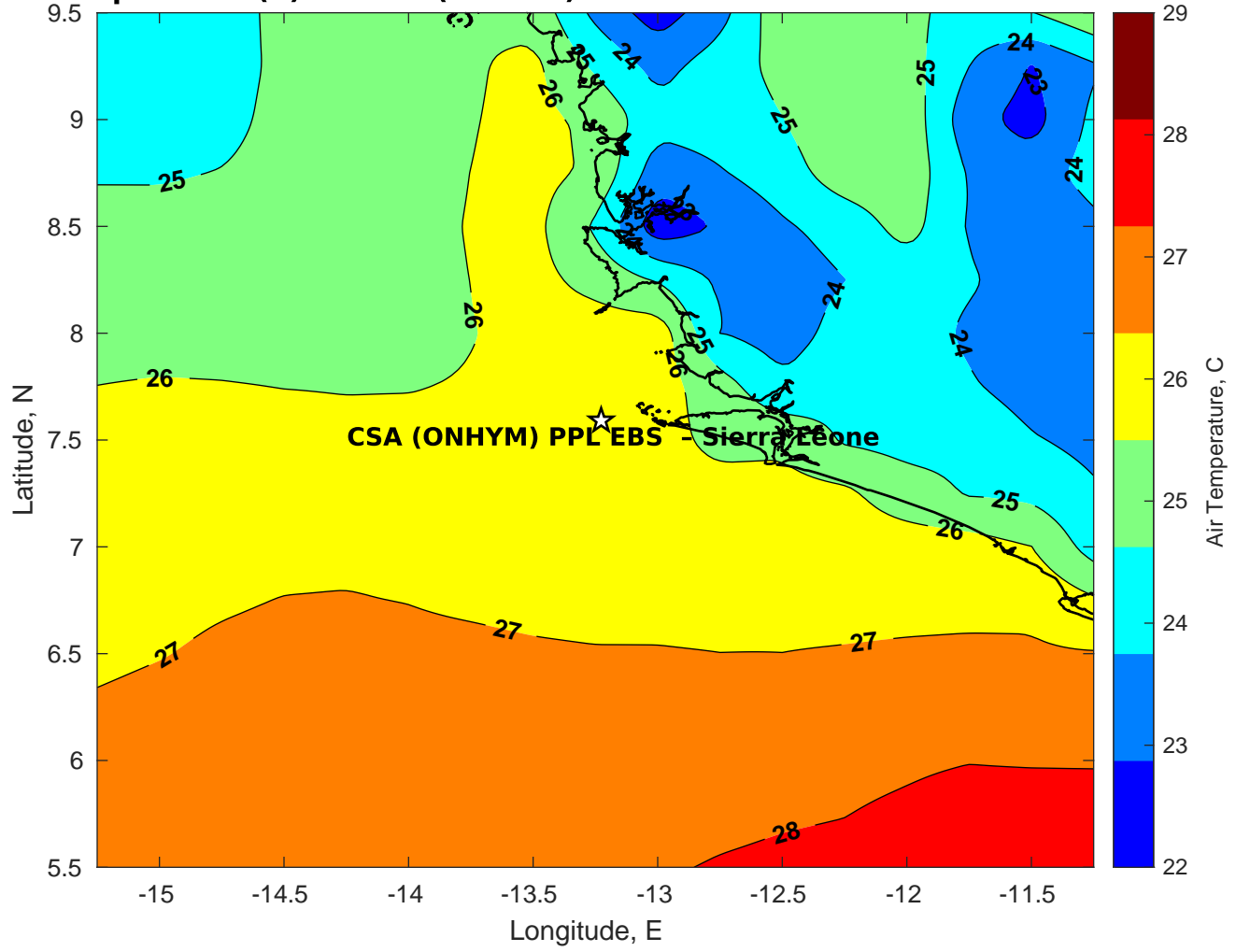
Air Temperature (C) for CSA (ONHYM) PPL EBS - Sierra Leone at 09-Mar-2025
