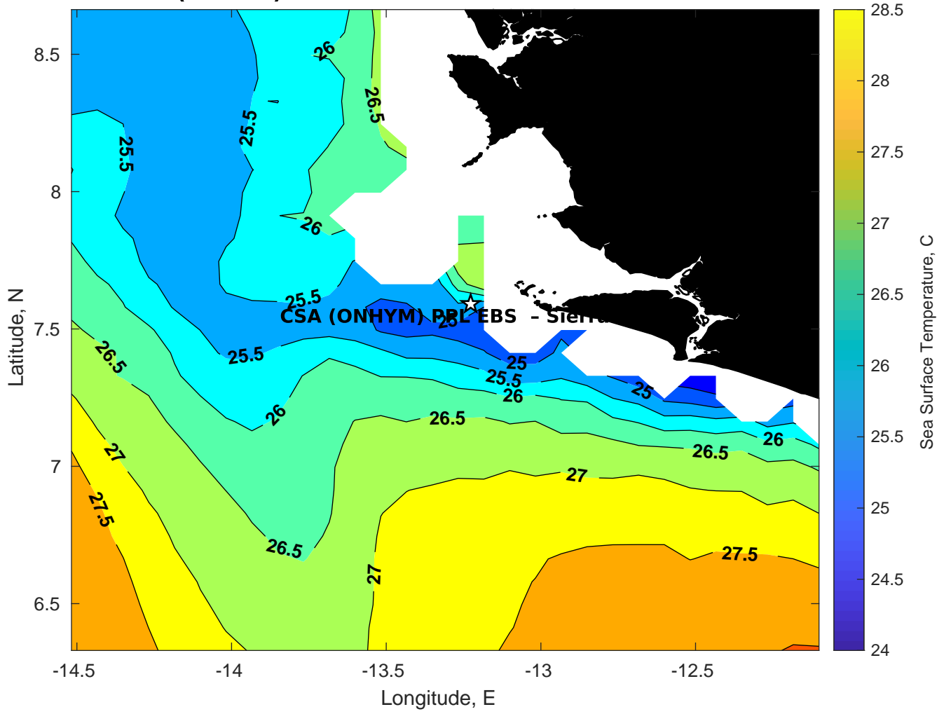
SST for CSA (ONHYM) PPL EBS - Sierra Leone at 08-Mar-2025 00:00:00
