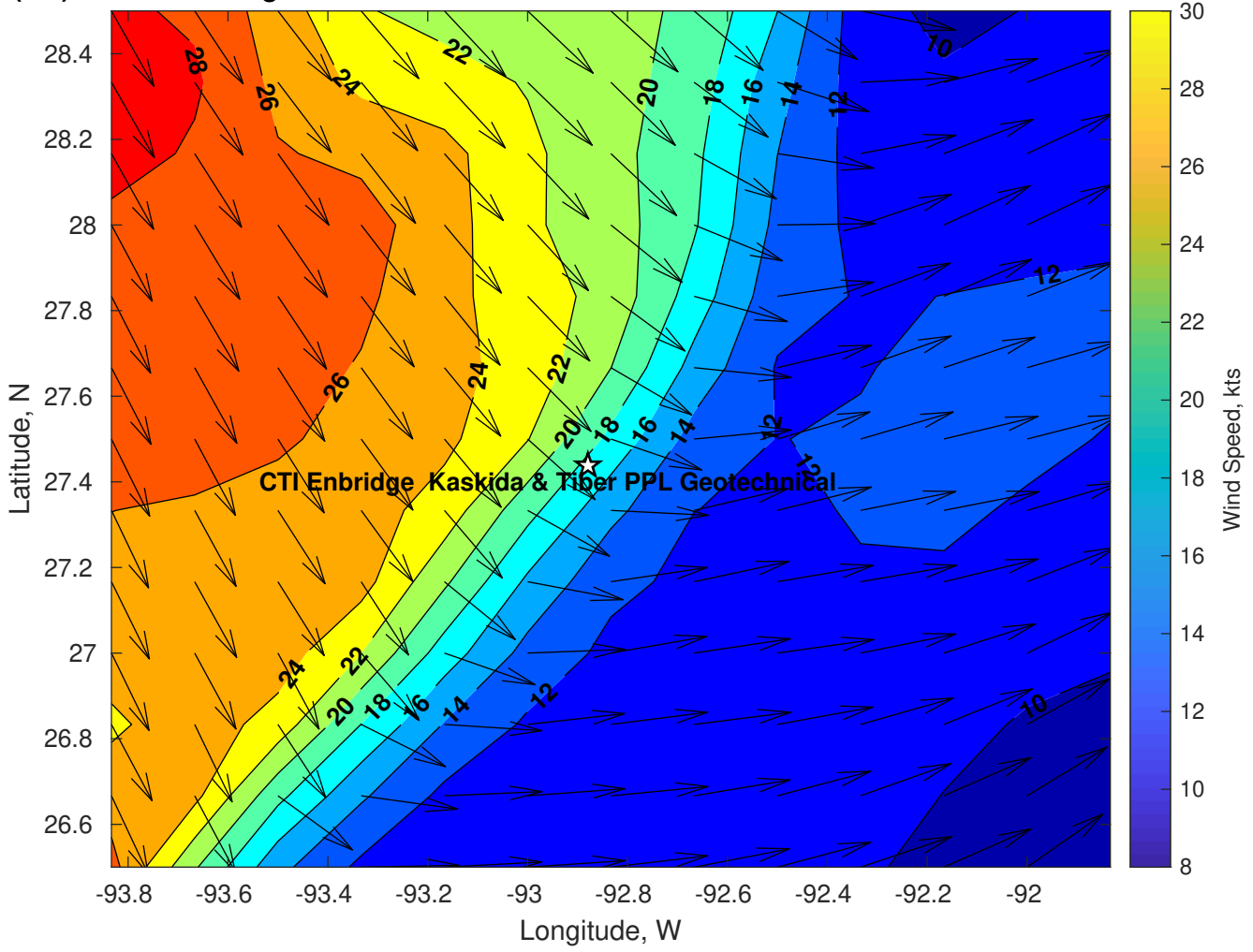
Winds (kts) for CTI Enbridge Kaskida & Tiber PPL Geotechnical at 09-Mar-2025 09:00:00
