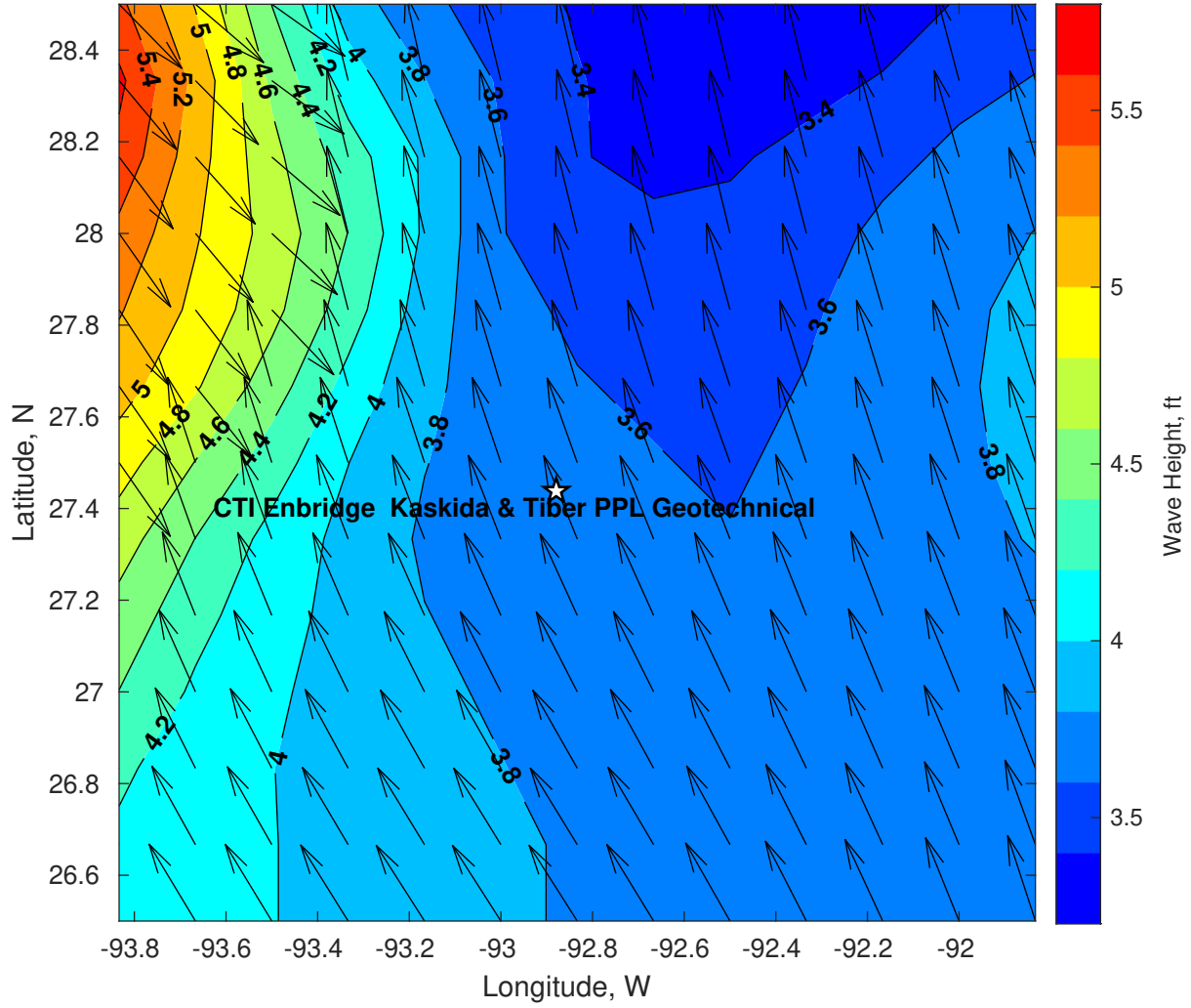
Wave Height (ft) for CTI Enbridge Kaskida & Tiber PPL Geotechnical at 09-Mar-2025 09:00:00
