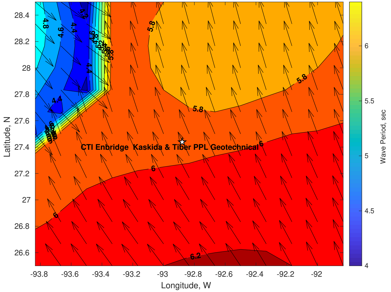
Wave Period (sec) for CTI Enbridge Kaskida & Tiber PPL Geotechnical at 09-Mar-2025 09:00:00
