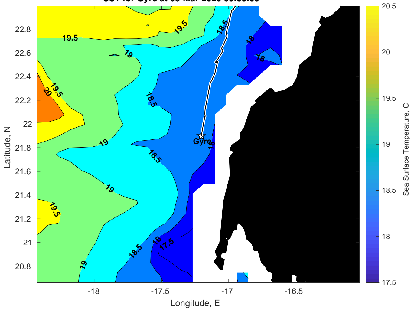
SST for Gyre at 08-Mar-2025 00:00:00
