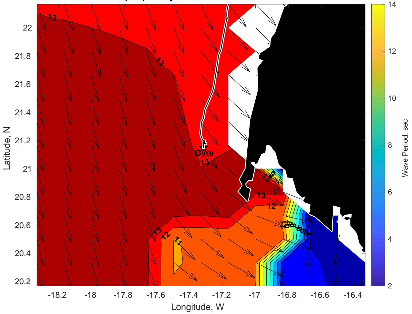
Wave Period (sec) for Gyre at 09-Mar-2025 09:00:00
