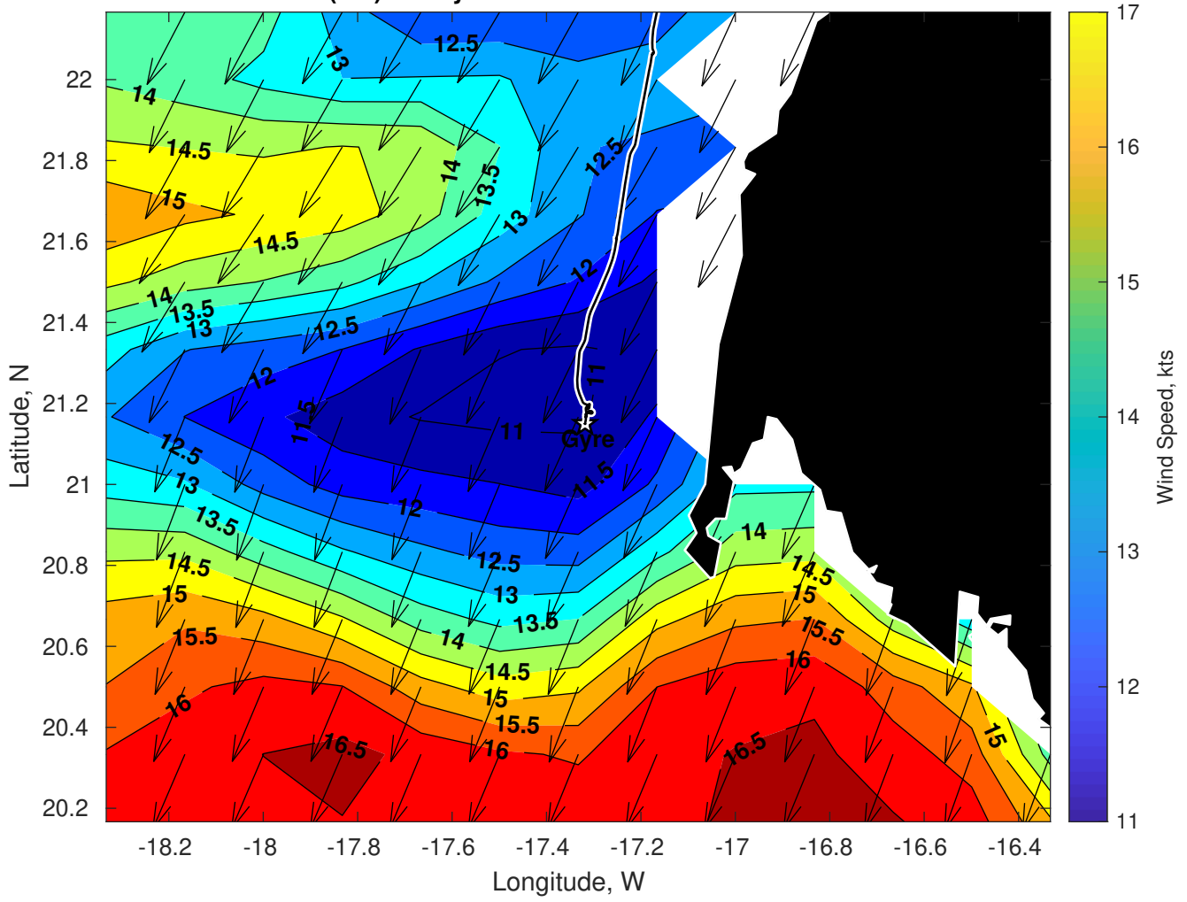
Winds (kts) for Gyre at 09-Mar-2025 09:00:00
