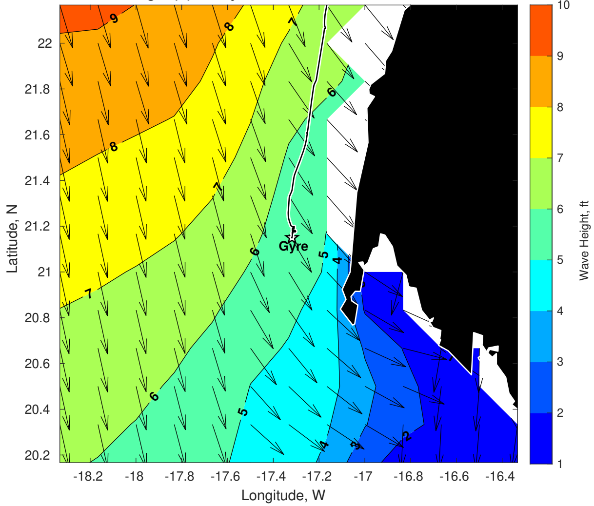
Wave Height (ft) for Gyre at 09-Mar-2025 09:00:00
