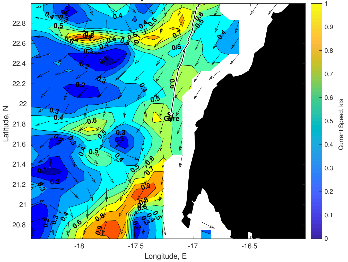
Surface Currents for Gyre at 08-Mar-2025 00:00:00
