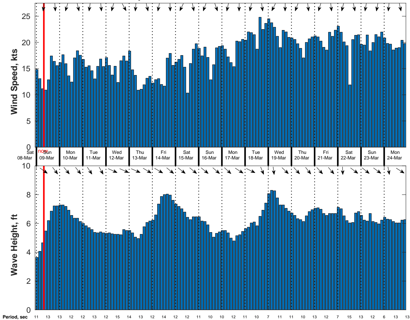
Wind & Wave Forecast for Gyre from 08-Mar-2025 23:00:00 to 24-Mar-2025 23:00:00
